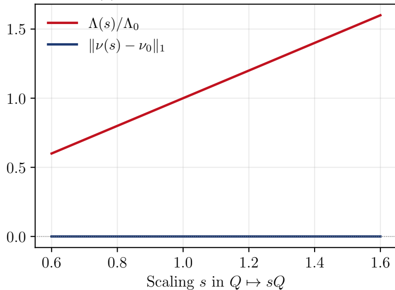
(a) Scaling gauge: \Lambda moves, \nu fixed
