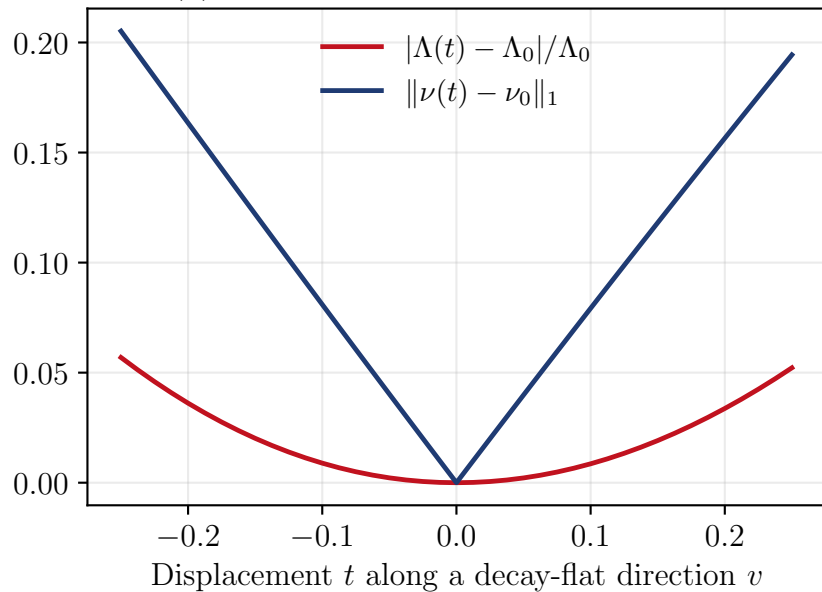
(b) Decay-flat direction: \nu moves, \Lambda fixed
