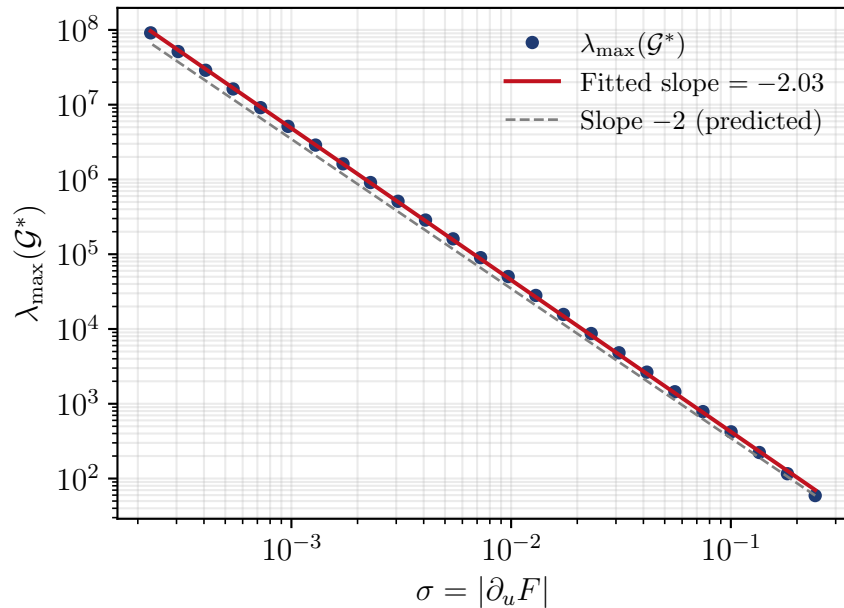
(b) Rank-one fold divergence, \mathcal{G}^* \sim \sigma^{-2}
