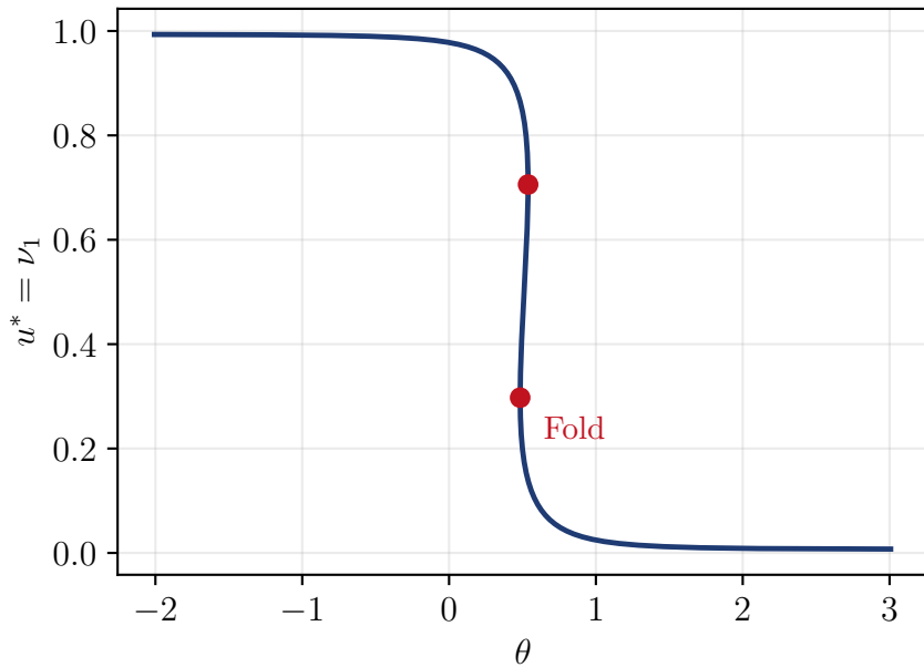
(a) Self-consistency curve F(\theta, u) = \nu_1 - u = 0
