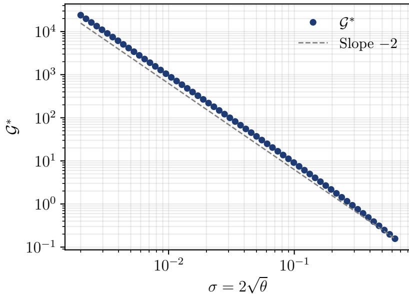
(b) \mathcal{G}^* \sim \sigma^{-2} (fitted slope -2.01 )
