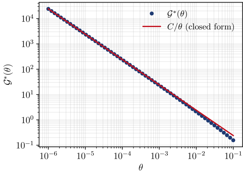
(a) \mathcal{G}^* \sim C/\theta (fitted slope -1.01 )
