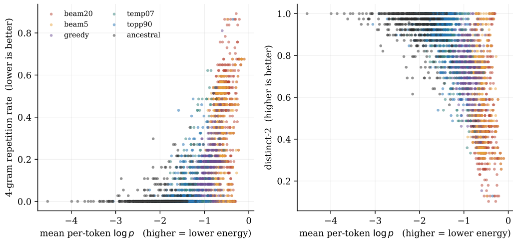
Figure 11: Mean per-token log-probability against 4-gram repetition rate and distinct-2 diversity for GPT-2 Large, one point per generation, coloured by decoding strategy. This figure supports Section 5.7.
