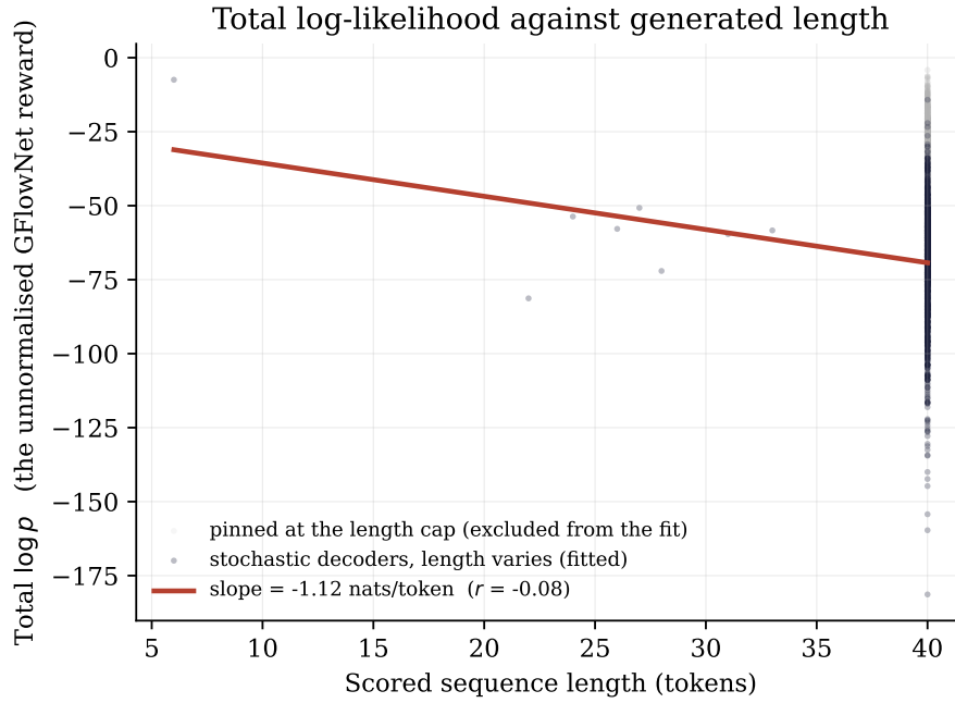
Figure 13: Total log-likelihood against generated length for GPT-2 Large. The regression is fitted over the three stochastic decoders (ancestral, top- p , temperature), where length varies, giving a slope of -1.12 nats per token; the deterministic decoders pinned at the length cap carry no length information and are shown faintly but excluded from the fit. This figure supports Section 5.7 and Section 5.10, where the slope and its censoring caveat are discussed.
