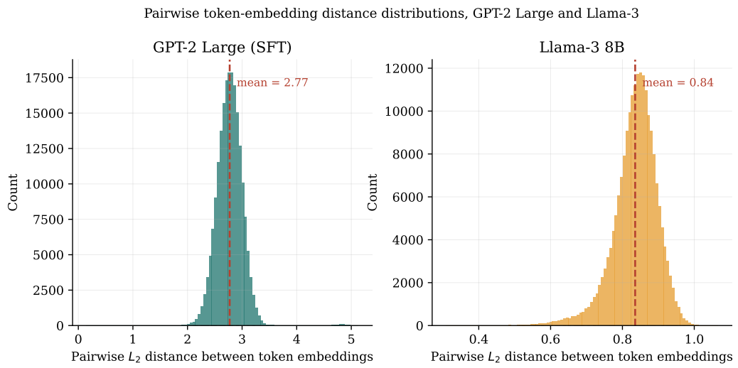
Figure 12: Distributions of pairwise token-embedding distances in GPT-2 Large and Llama-3, plotted on separate scales. This figure supports Section 5.8.
