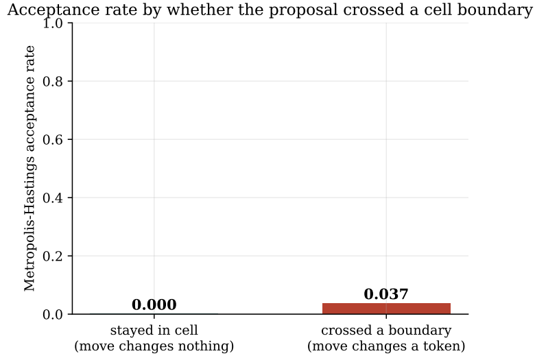
Figure 10: Metropolis-Hastings acceptance rate for the continuous policy sampler with gradient normalization off and the correction enabled (configuration cls_policy_gnoff_mh ), conditioned on whether the proposal crossed a Voronoi cell boundary. Within-cell moves are accepted essentially never and boundary crossings only 3.7% of the time. This figure supports Section 5.3.
