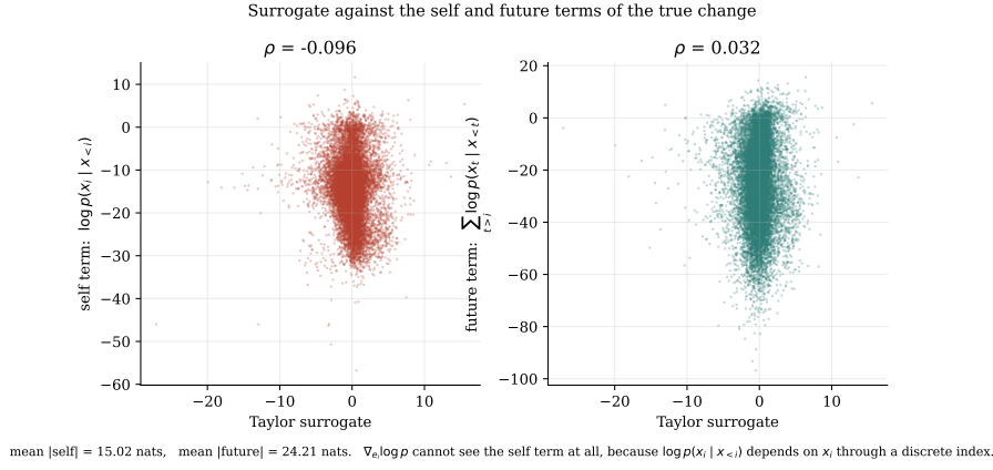
Figure 8: The true energy change decomposed into its self term and its future term, each plotted against the gradient surrogate, for GPT-2 Large. This figure supports Section 5.6.
