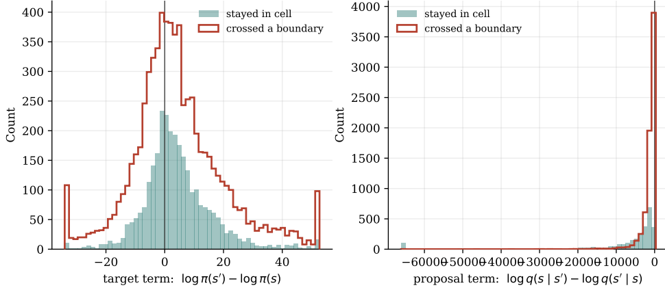
Figure 4: Decomposition of the Metropolis-Hastings acceptance ratio in the continuous sampler, for proposals that stay within a Voronoi cell against those that cross a boundary. Left: the target log-ratio. Right: the proposal log-ratio. Both on a log-probability scale.
