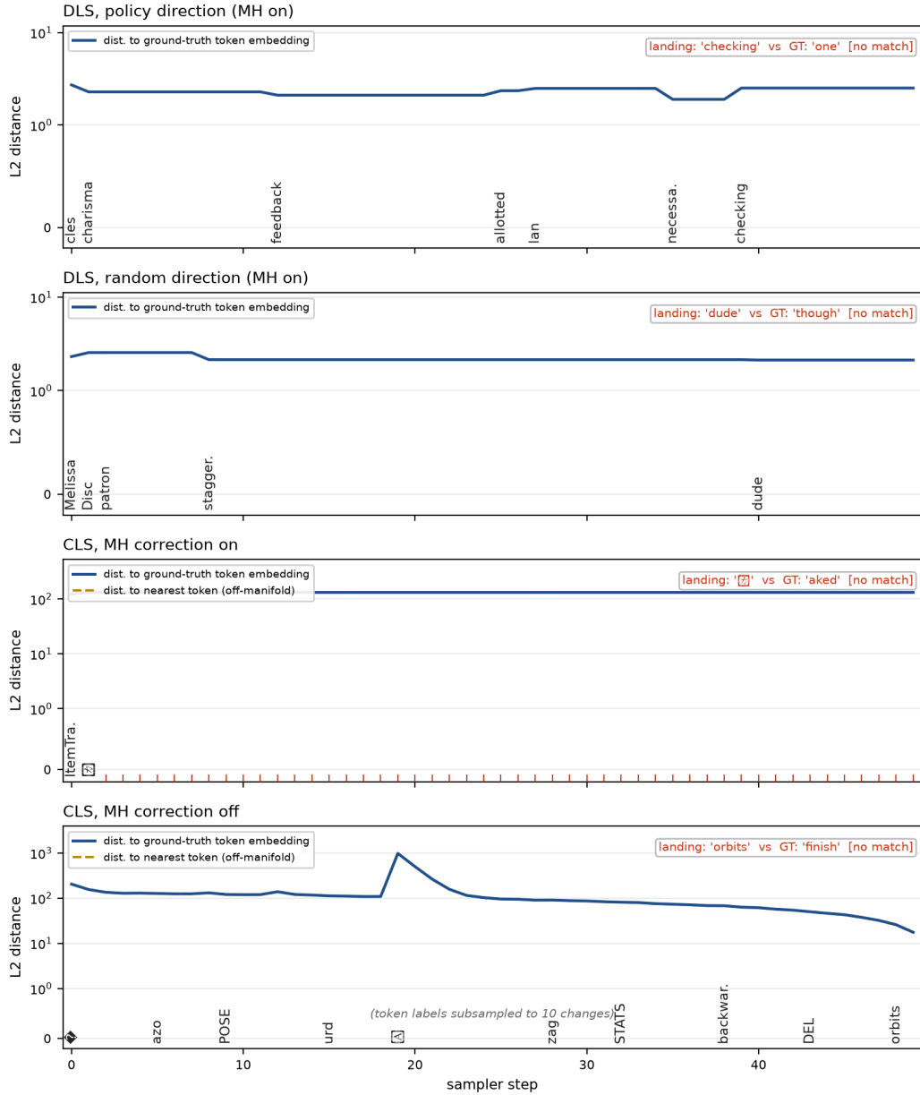
Figure 14: Full-space distances along the sampling trajectory for one seeded trace, index 5, on a symmetric-log axis, one panel per configuration. Solid line: L_2 distance to the ground-truth token embedding. Dashed line, continuous sampler only: L_2 distance to the nearest token of any kind. Red ticks mark rejected proposals. The discrete sampler's nearest-token distance is identically zero and is therefore not drawn.
