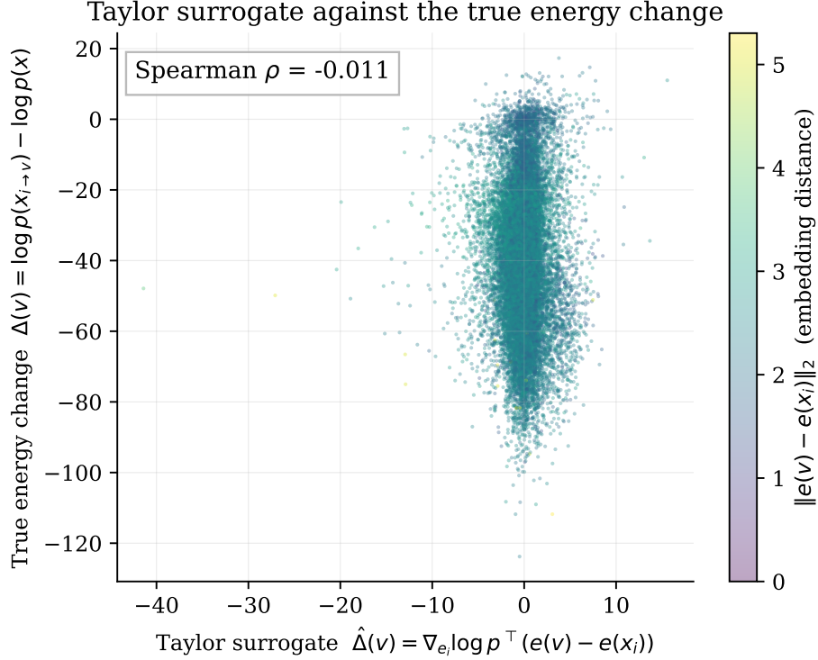
Figure 5: The first-order Taylor surrogate used by the discrete proposal, plotted against the true change in sequence log-likelihood for GPT-2 Large, coloured by the embedding distance of the candidate token. n = 400,000 candidate–sequence pairs.
