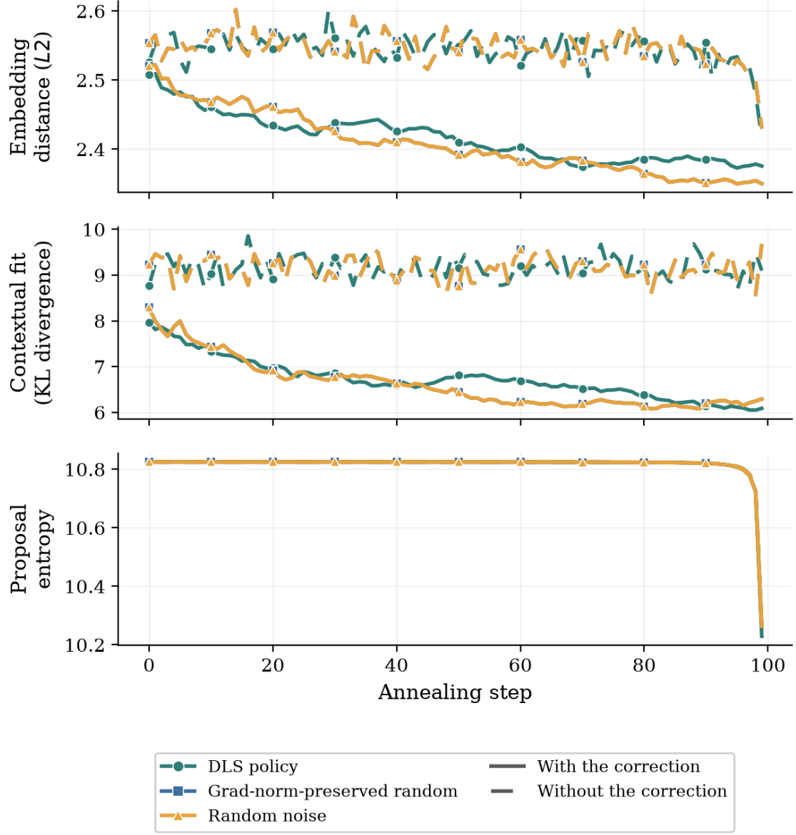
Figure 2: Discrete Langevin Sampler trajectories on GPT-2 Large over a 100-step annealing schedule, averaged across sequences. Panels, axes, line styles and markers as in Figure 1.
