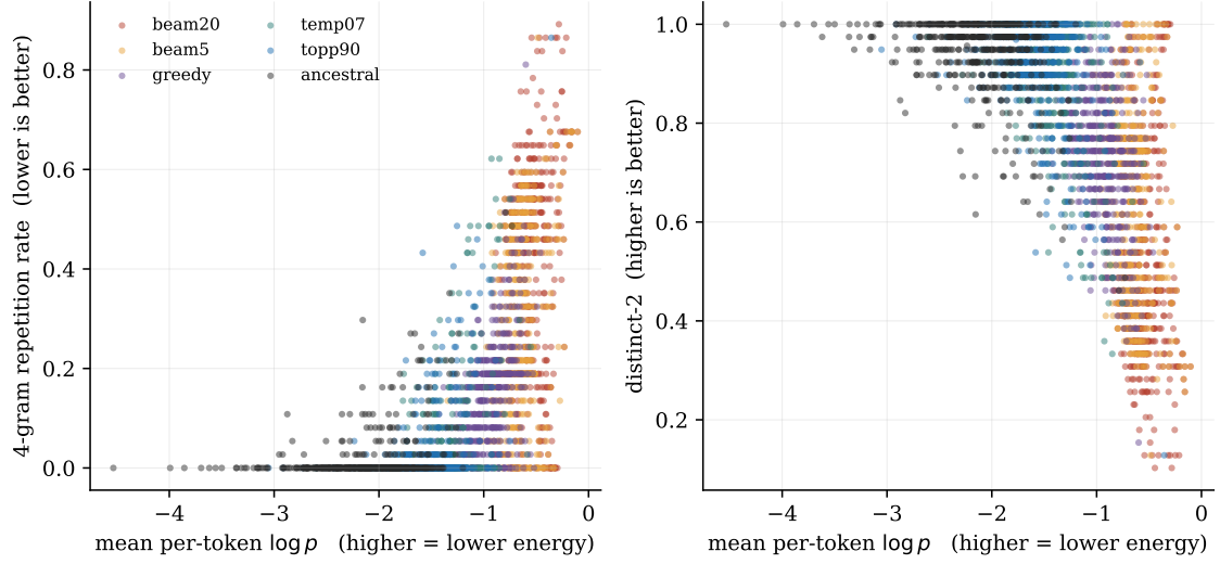
Figure 9: Mean per-token log-probability against 4-gram repetition rate and distinct-2 diversity for GPT-2 Large, one point per generation, coloured by decoding strategy. This figure supports Section 5.7.
