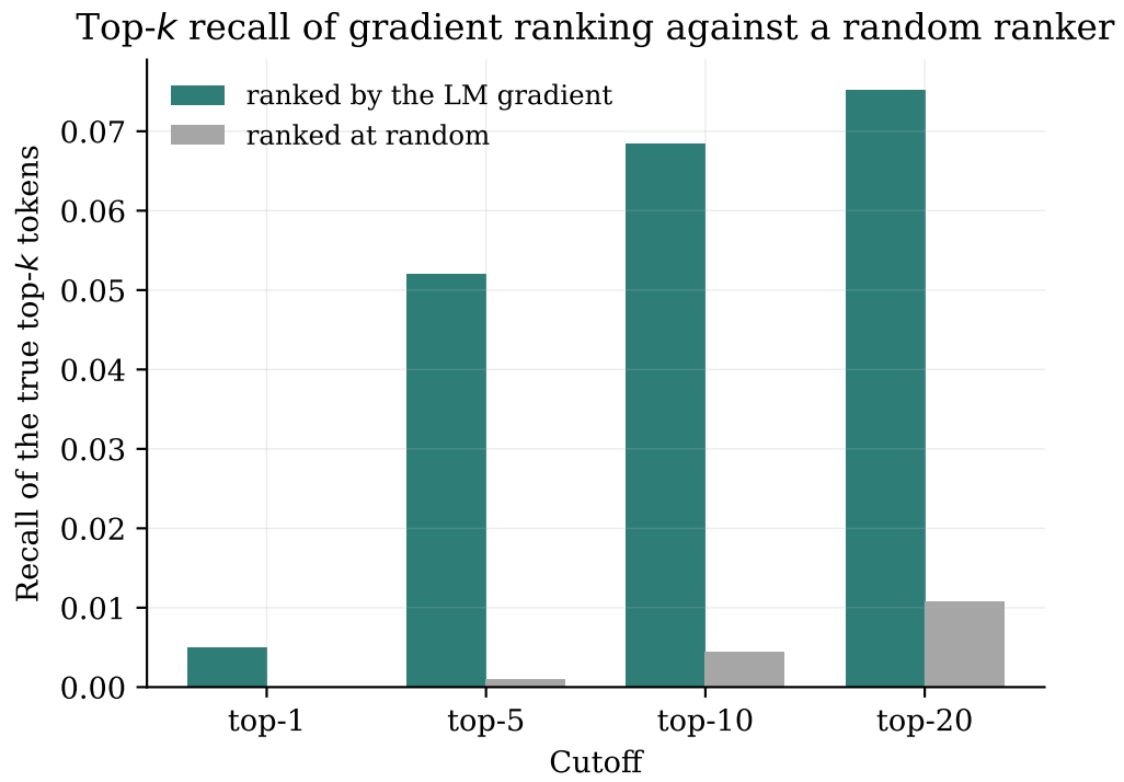
Figure 7: Recall of the true top- k token substitutions by the gradient-ranked top- k , against a random-ranking baseline, for GPT-2 Large. This figure supports Section 5.4.
