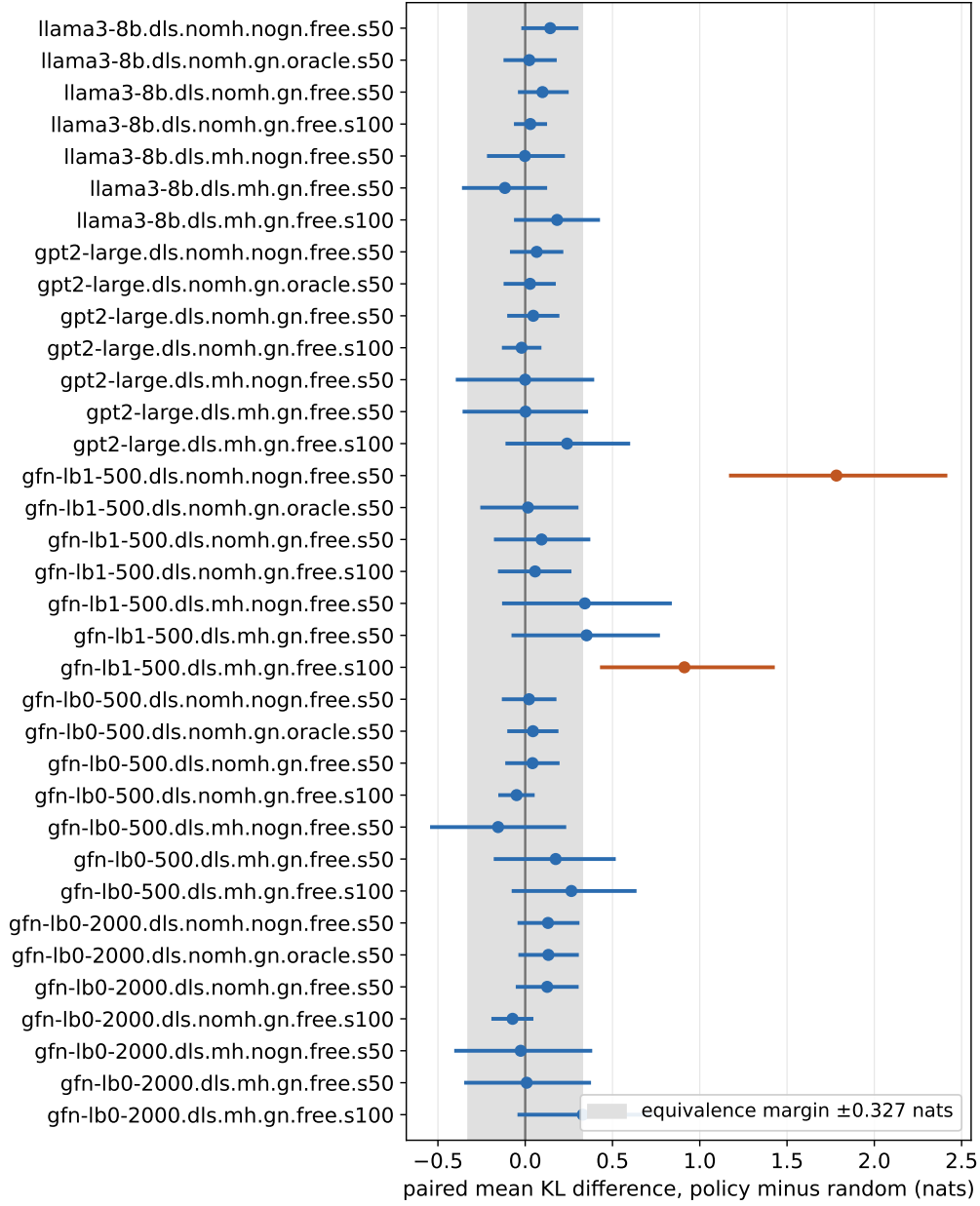
Figure 3: Paired difference in chain-mean KL, policy minus norm-matched random direction, for every configuration in the grid with both arms present (35 configurations). Points are paired means, bars are 95% percentile-bootstrap intervals over n = 200 paired sequences each, and the shaded band is the equivalence margin of \pm 0.327 nats, fixed in advance of the comparison. Intervals whose bounds exclude zero are drawn in the darker colour.
