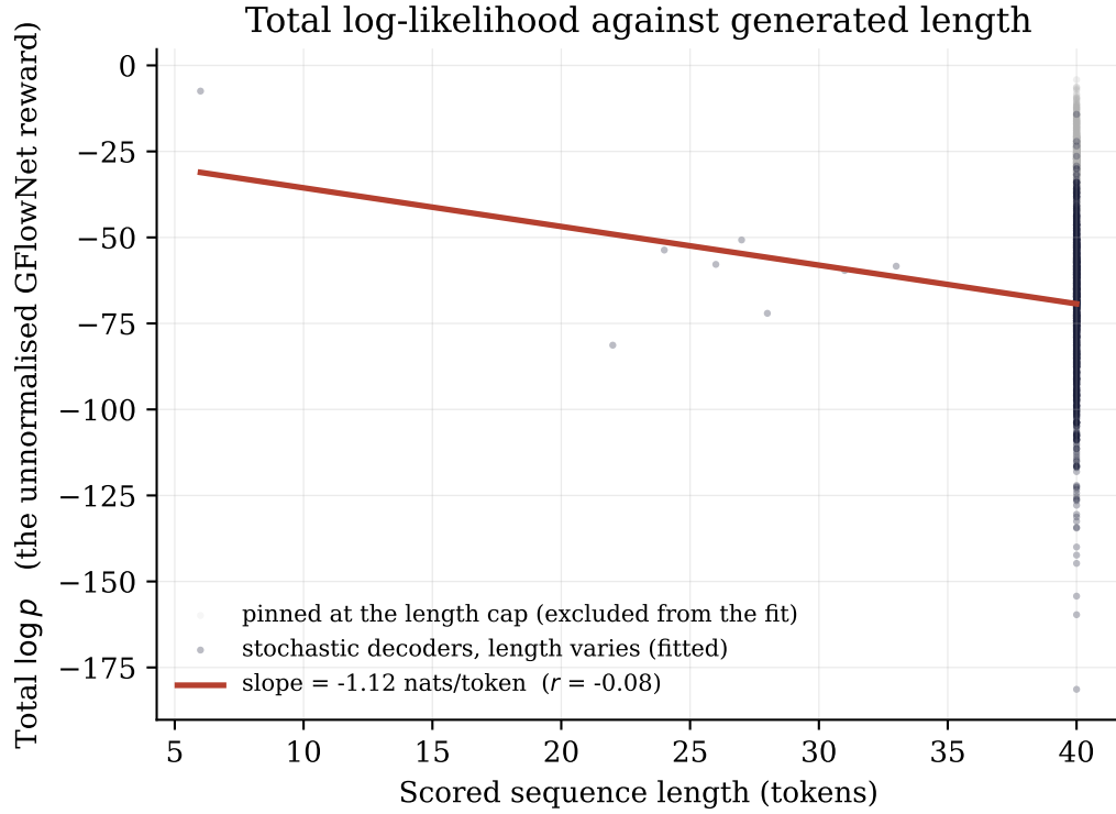
Figure 11: Total log-likelihood against generated length for GPT-2 Large. The regression is fitted over the three stochastic decoders (ancestral, top- p , temperature), where length varies, giving a slope of -1.12 nats per token; the deterministic decoders pinned at the length cap carry no length information and are shown faintly but excluded from the fit. This figure supports Section 5.7 and Section 5.9, where the slope and its censoring caveat are discussed.
