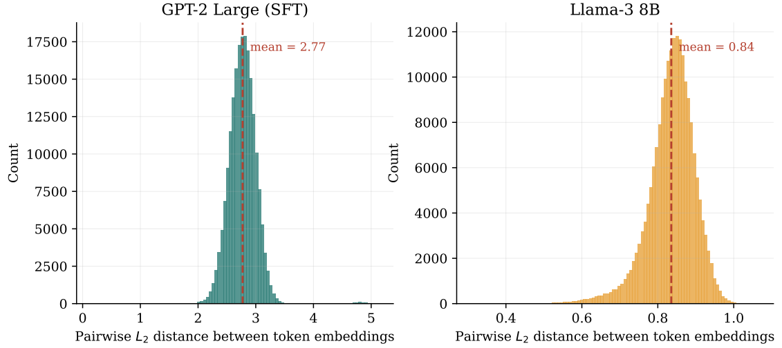
Figure 10: Distributions of pairwise token-embedding distances in GPT-2 Large and Llama-3, plotted on separate scales. This figure supports Section 5.8.
