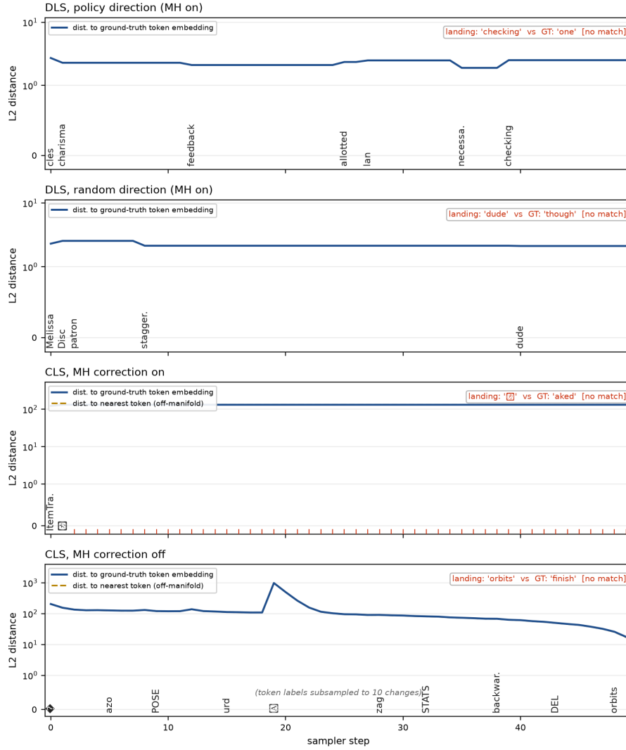
Figure 14: Full-space distances along the sampling trajectory for one seeded trace, index 5, on a symmetric-log axis, one panel per configuration. Solid line: L_2 distance to the ground-truth token embedding. Dashed line, continuous sampler only: L_2 distance to the nearest token of any kind. Red ticks mark rejected proposals. The discrete sampler's nearest-token distance is identically zero and is therefore not drawn.
