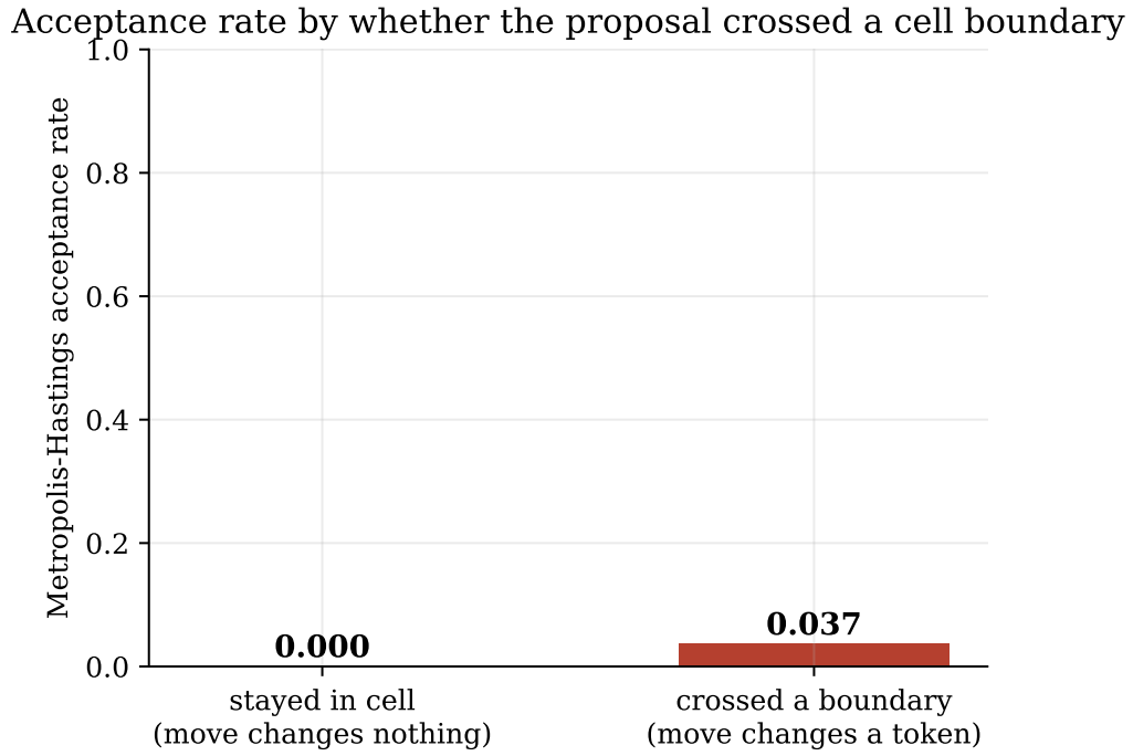
Figure 8: Metropolis–Hastings acceptance rate for the continuous policy sampler with gradient normalization off and the correction enabled (configuration cls_policy_gnoff_mh ), conditioned on whether the proposal crossed a Voronoi cell boundary. Within-cell moves are accepted essentially never and boundary crossings only 3.7% of the time. This figure supports Section 5.2.
