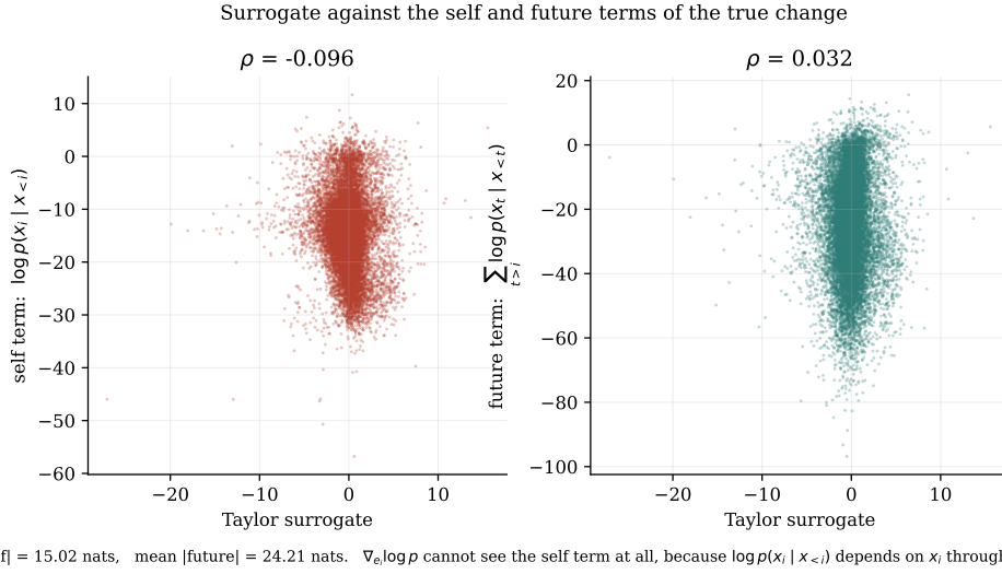
Figure 6: The true energy change decomposed into its self term and its future term, each plotted against the gradient surrogate, for GPT-2 Large. This figure supports Section 5.4.
