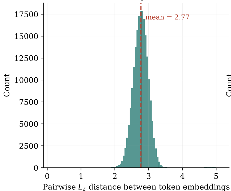
GPT-2 Large (SFT)
