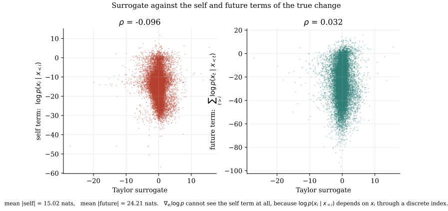
Figure A.1: The true energy change decomposed into its self term and its future term, each plotted against the gradient surrogate, for GPT-2 Large. This figure supports Section 5.6.
