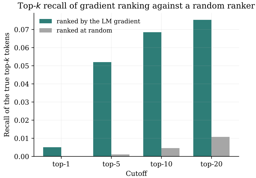
Figure A.2: Recall of the true top- k token substitutions by the gradient-ranked top- k , against a random-ranking baseline, for GPT-2 Large. This figure supports Section 5.6.
