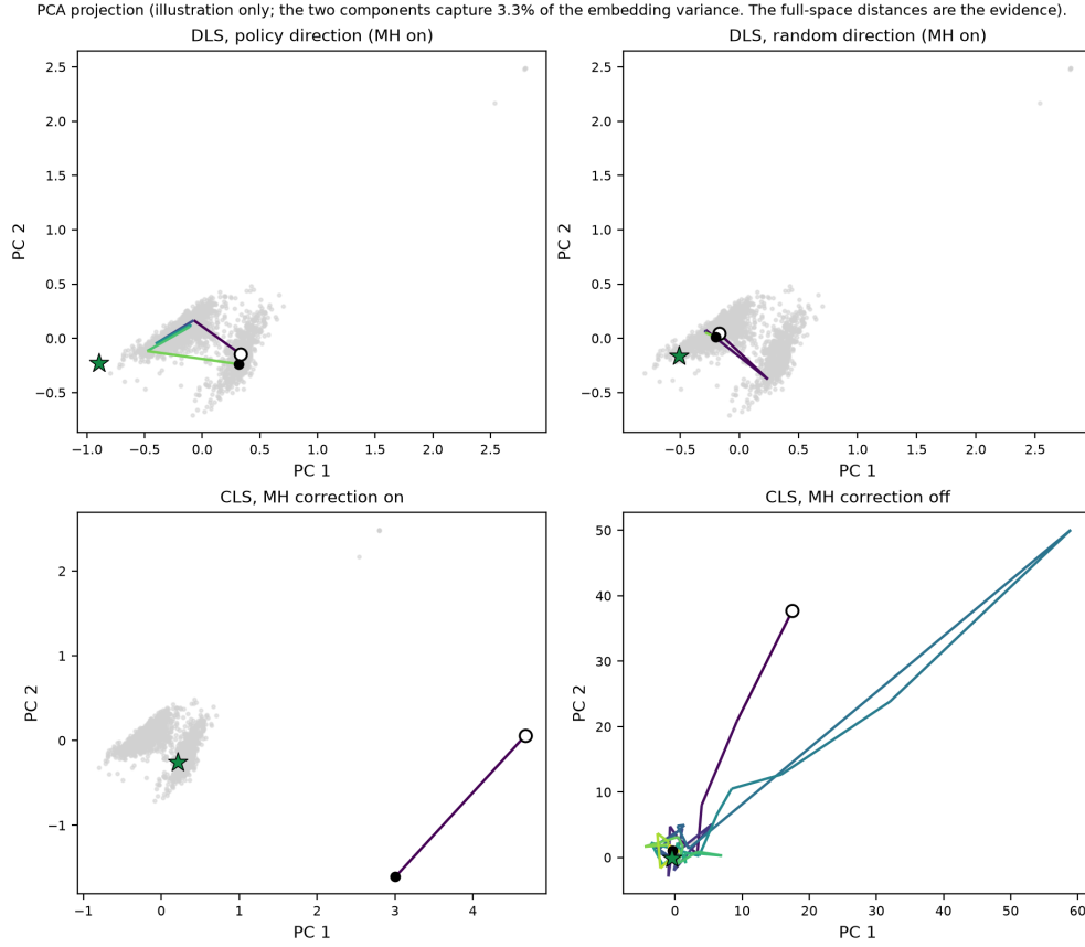
Figure A.8: PCA projection of the same seeded trace, one panel per configuration. Grey cloud: the vocabulary embeddings. Open circle: the start state. Filled dot: the end state. Star: the ground-truth token. The two components capture 3.3% of the embedding variance, so this projection is illustration only and the full-space distances of Figure A.7 carry the argument.
