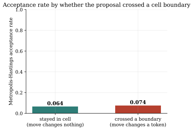
Figure A.3: Metropolis-Hastings acceptance rate in the continuous sampler, conditioned on whether the proposal crossed a Voronoi cell boundary. This figure supports Section 5.3.
