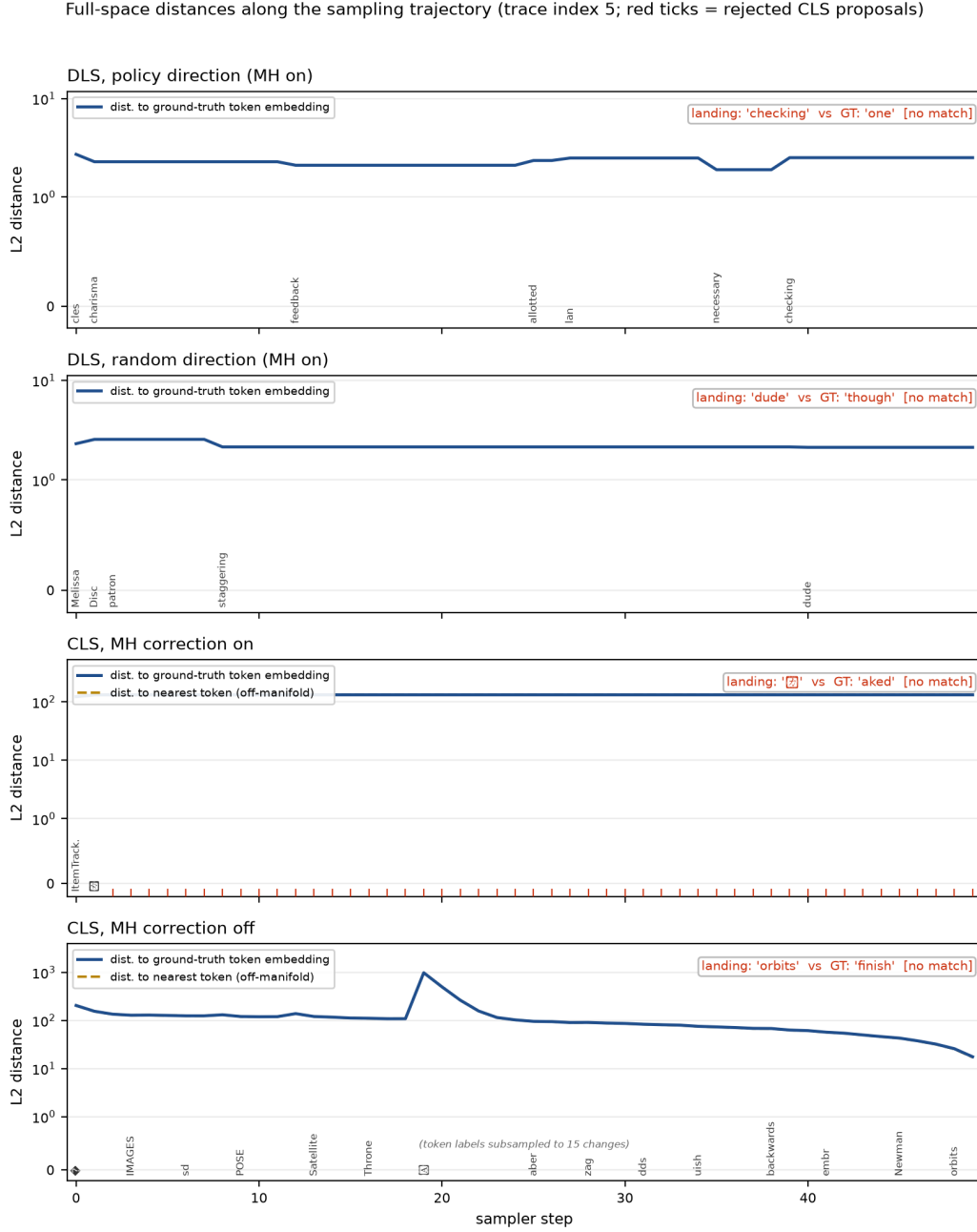
Figure A.7: Full-space distances along the sampling trajectory for one seeded trace, index 5, on a symmetric-log axis, one panel per configuration. Solid line: L_2 distance to the ground-truth token embedding. Dashed line, continuous sampler only: L_2 distance to the nearest token of any kind. Red ticks mark rejected proposals. The discrete sampler’s nearest-token distance is identically zero and is therefore not drawn.
