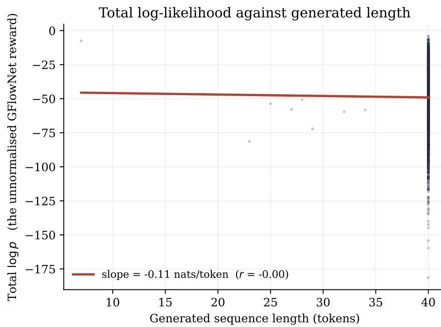
Figure A.6: Total log-likelihood against generated length for GPT-2 Large, with the fitted regression line. This figure supports Section 5.7 and Section 5.10, where the slope and its censoring caveat are discussed.
