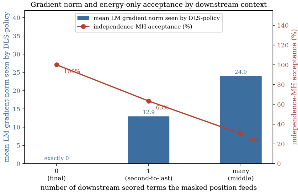
Figure 5.6: The final-position experiment against the number of downstream scored terms. Left axis, bars: the mean language-model gradient norm the discrete sampler consumes. Right axis, line: the independence sampler’s acceptance rate.
