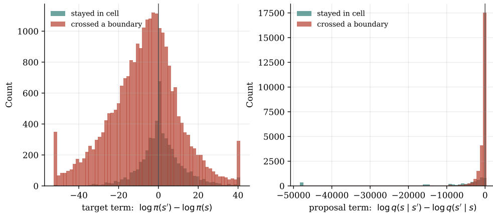
Figure 5.3: Decomposition of the Metropolis-Hastings acceptance ratio in the continuous sampler, for proposals that stay within a Voronoi cell against those that cross a boundary. Left: the target log-ratio. Right: the proposal log-ratio. Both on a log-probability scale.
