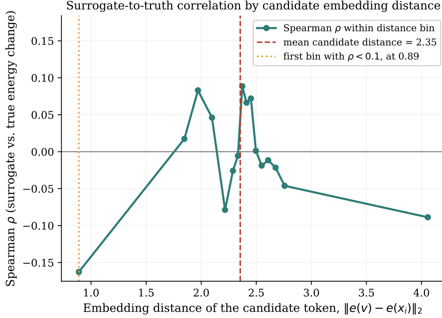
Figure 5.5: Correlation between the gradient surrogate and the true energy change as a function of the embedding distance of the candidate token, for GPT-2 Large. Dashed line: the mean linearization-candidate distance, 2.35. Dotted line: the smallest binned distance at which the correlation falls below 0.1.
