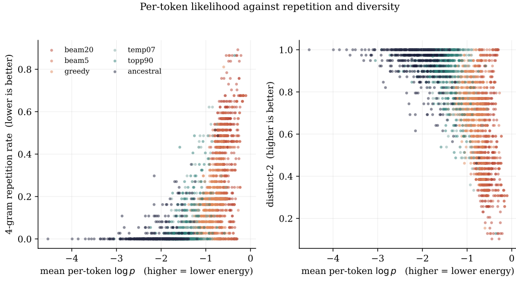
Figure A.4: Mean per-token log-probability against 4-gram repetition rate and distinct-2 diversity for GPT-2 Large, one point per generation, coloured by decoding strategy. This figure supports Section 5.7.
