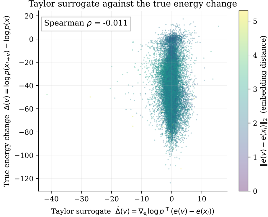
Figure 5.4: The first-order Taylor surrogate used by the discrete proposal, plotted against the true change in sequence log-likelihood for GPT-2 Large, coloured by the embedding distance of the candidate token. n = 400,000 candidate-sequence pairs.
