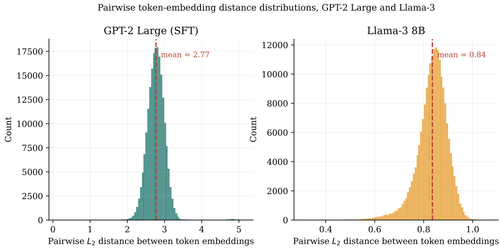
Figure A.5: Distributions of pairwise token-embedding distances in GPT-2 Large and Llama-3, plotted on separate scales. This figure supports Section 5.8.
