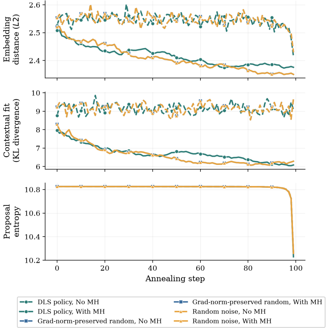
Figure 5.2: Discrete Langevin Sampler trajectories on GPT-2 Large over a 100-step annealing schedule, averaged across sequences. Panels, axes, line styles and markers as in Figure 5.1.
