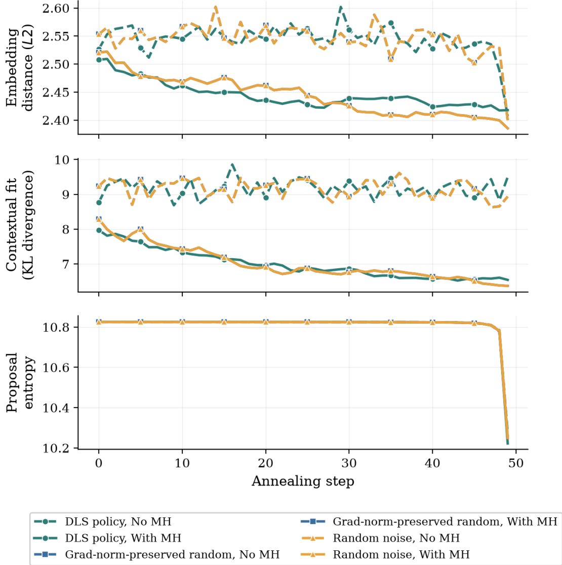
Figure 5.1: Discrete Langevin Sampler trajectories on GPT-2 Large over a 50-step annealing schedule, averaged across sequences. Panels, top to bottom: embedding distance, contextual fit measured by KL divergence, and proposal entropy. Solid lines are runs with the Metropolis-Hastings correction, dashed lines without it. Marker shape distinguishes the three proposal methods where their curves coincide.
