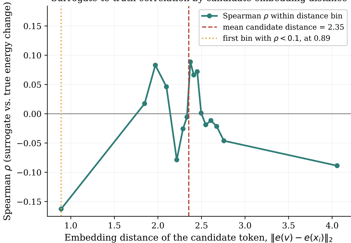
Surrogate-to-truth correlation by candidate embedding distance
