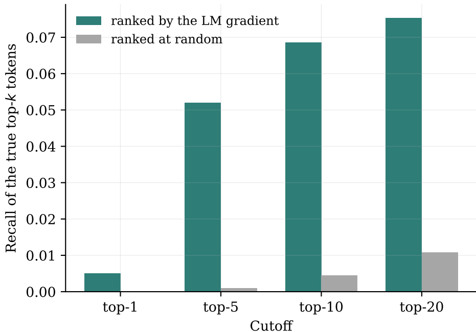
Top- k recall of gradient ranking against a random ranker
