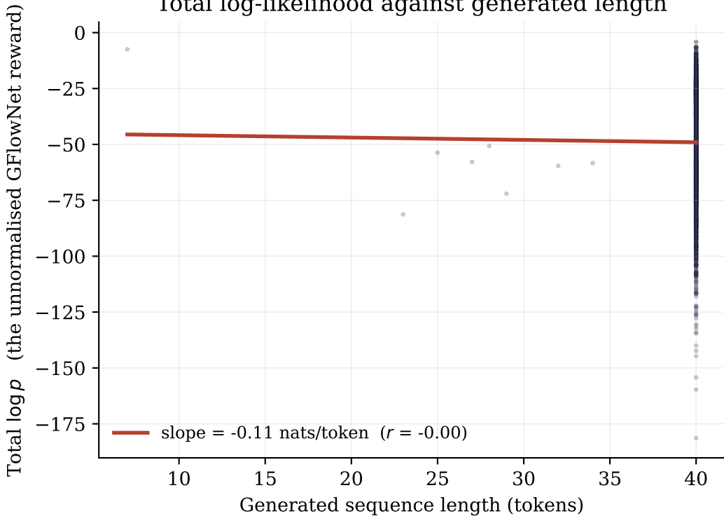
Total log-likelihood against generated length
