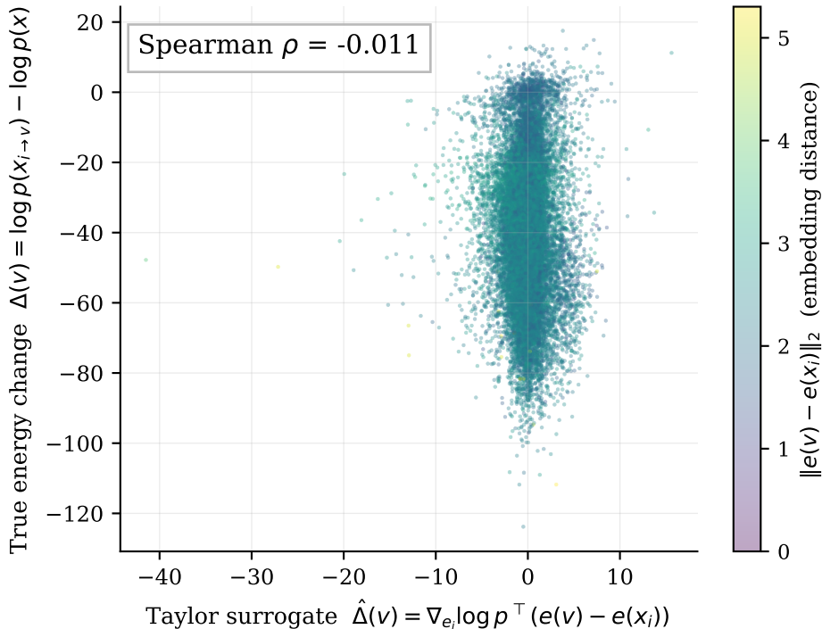
Taylor surrogate against the true energy change
