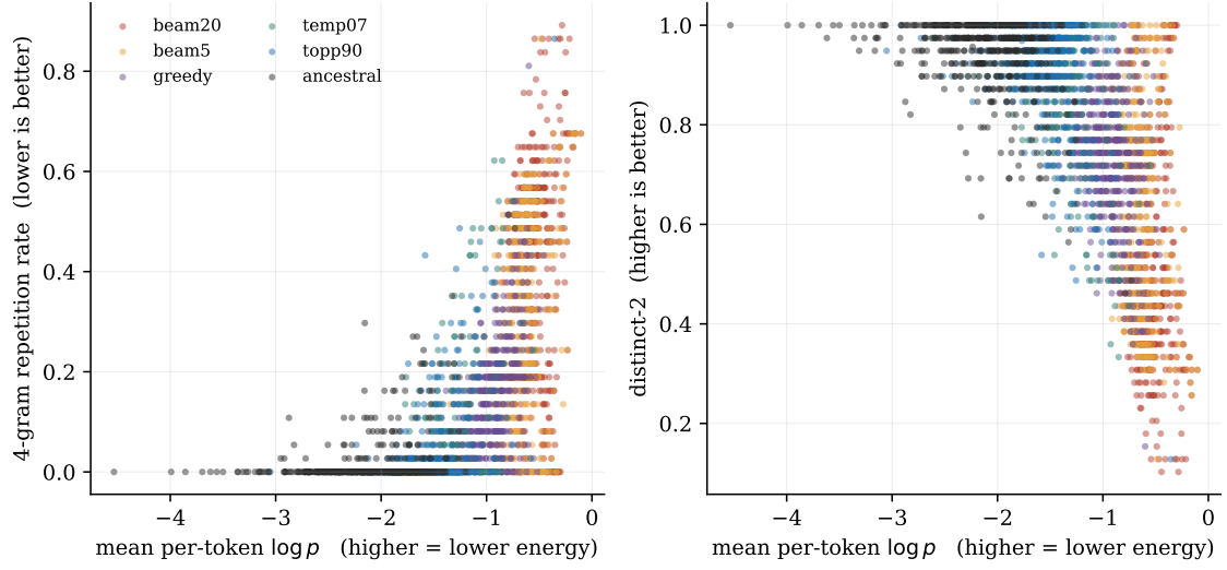
Figure 9: Mean per-token log-probability against 4-gram repetition rate and distinct-2 diversity for GPT-2 Large, one point per generation, coloured by decoding strategy.
