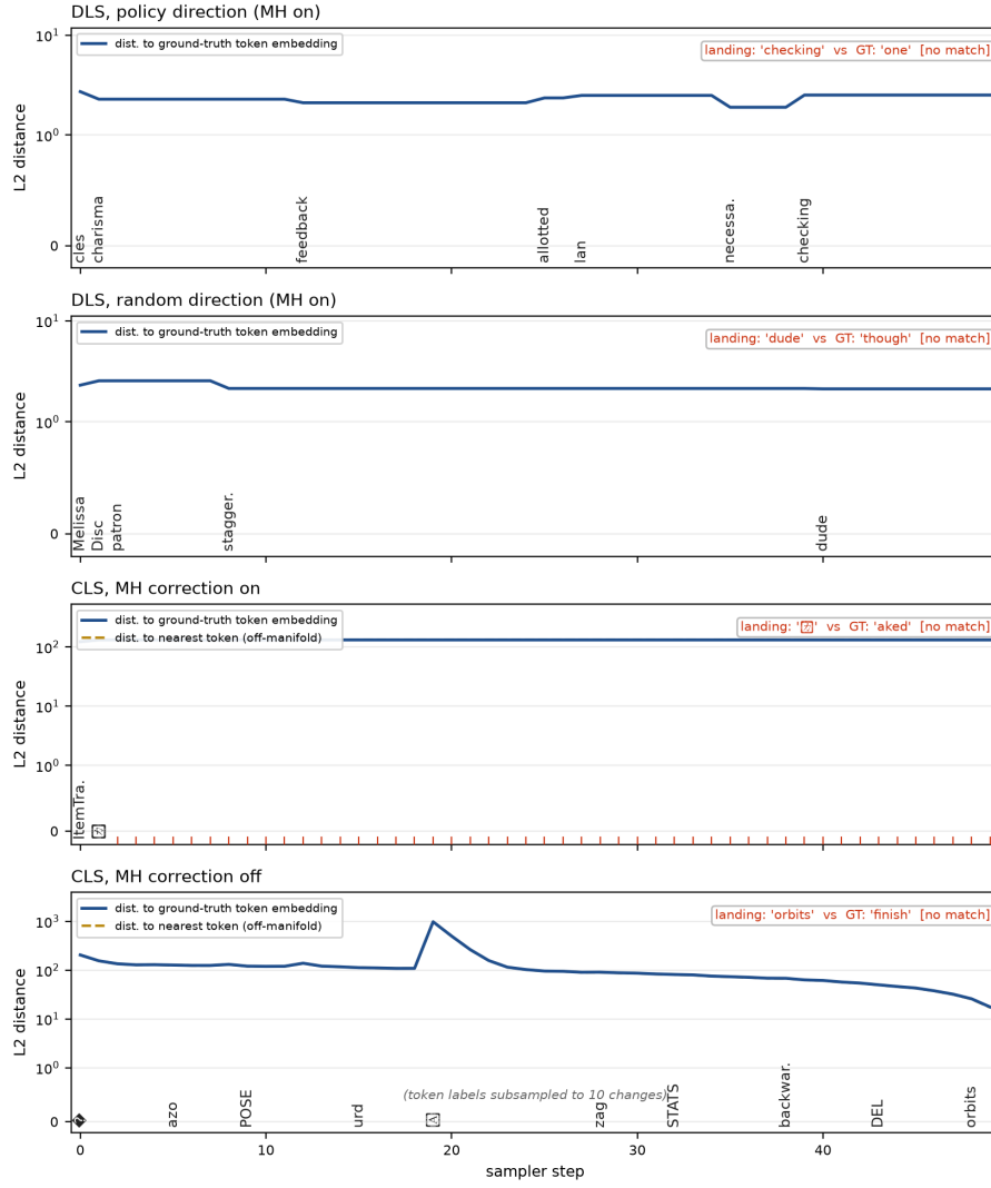
Figure 14: Full-space distances along the sampling trajectory for one trace, index 5, one panel per configuration.
