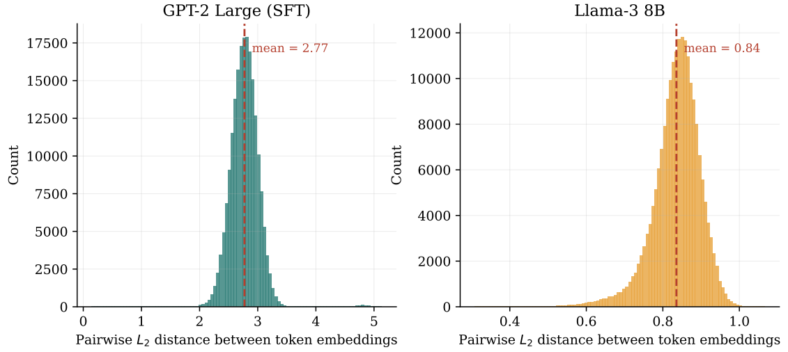
Figure 10: Distributions of pairwise token-embedding distances in GPT-2 Large and Llama-3, plotted on separate scales.
