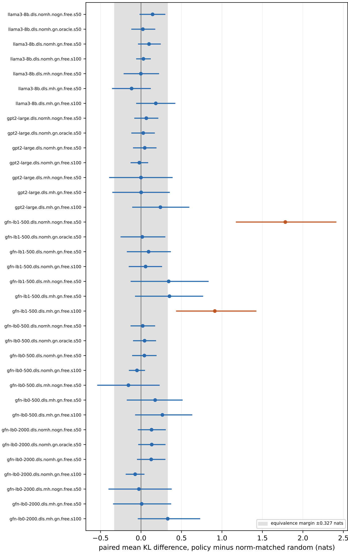
Paired policy minus norm-matched random direction, chain mean KL over the second half of the sc
