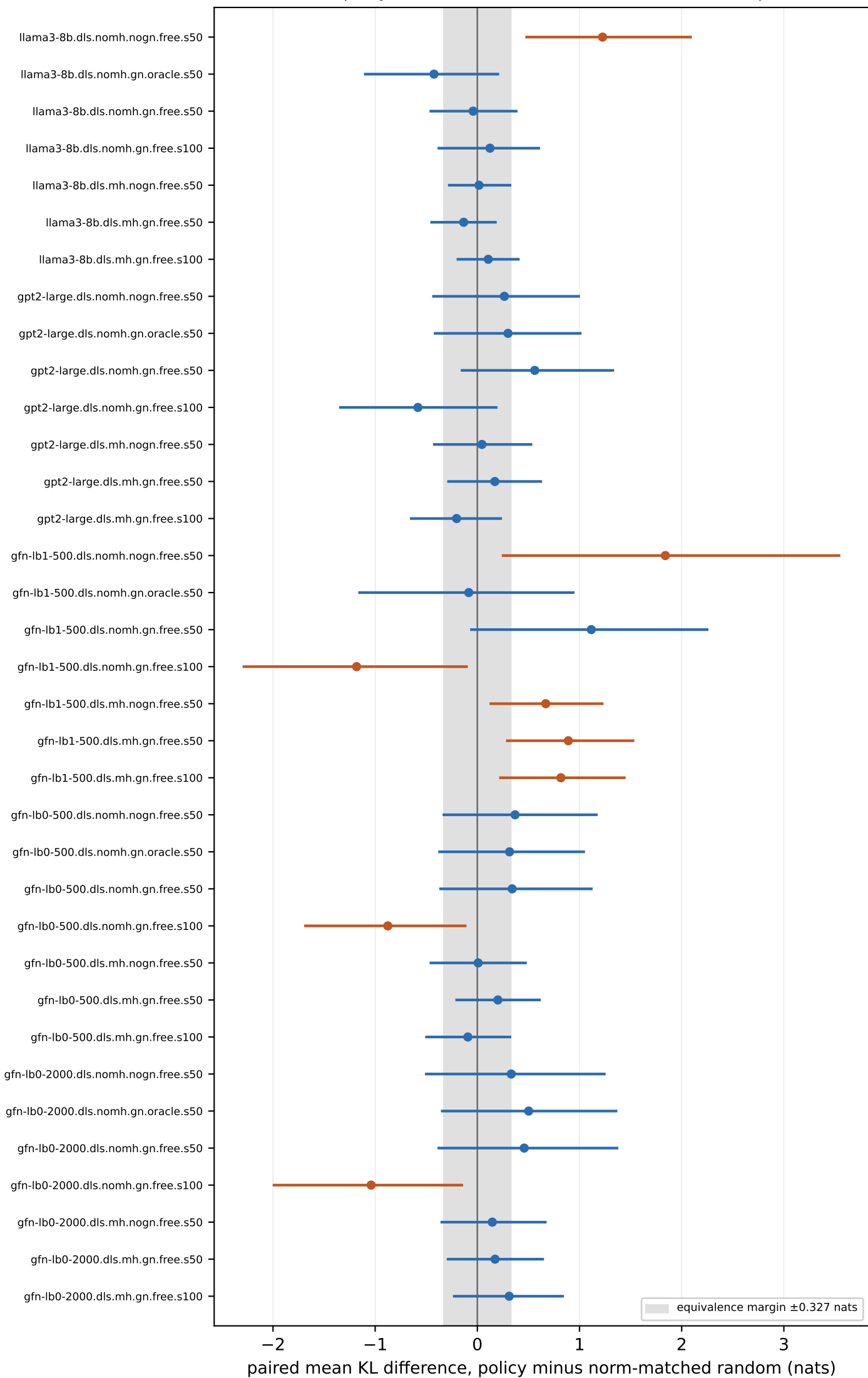
Paired policy minus norm-matched random direction, final-step KL
