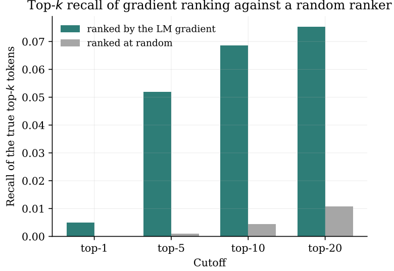
Figure 7: Recall of the true top- k token substitutions by the gradient-ranked top- k , against a random-ranking baseline, for GPT-2 Large.
