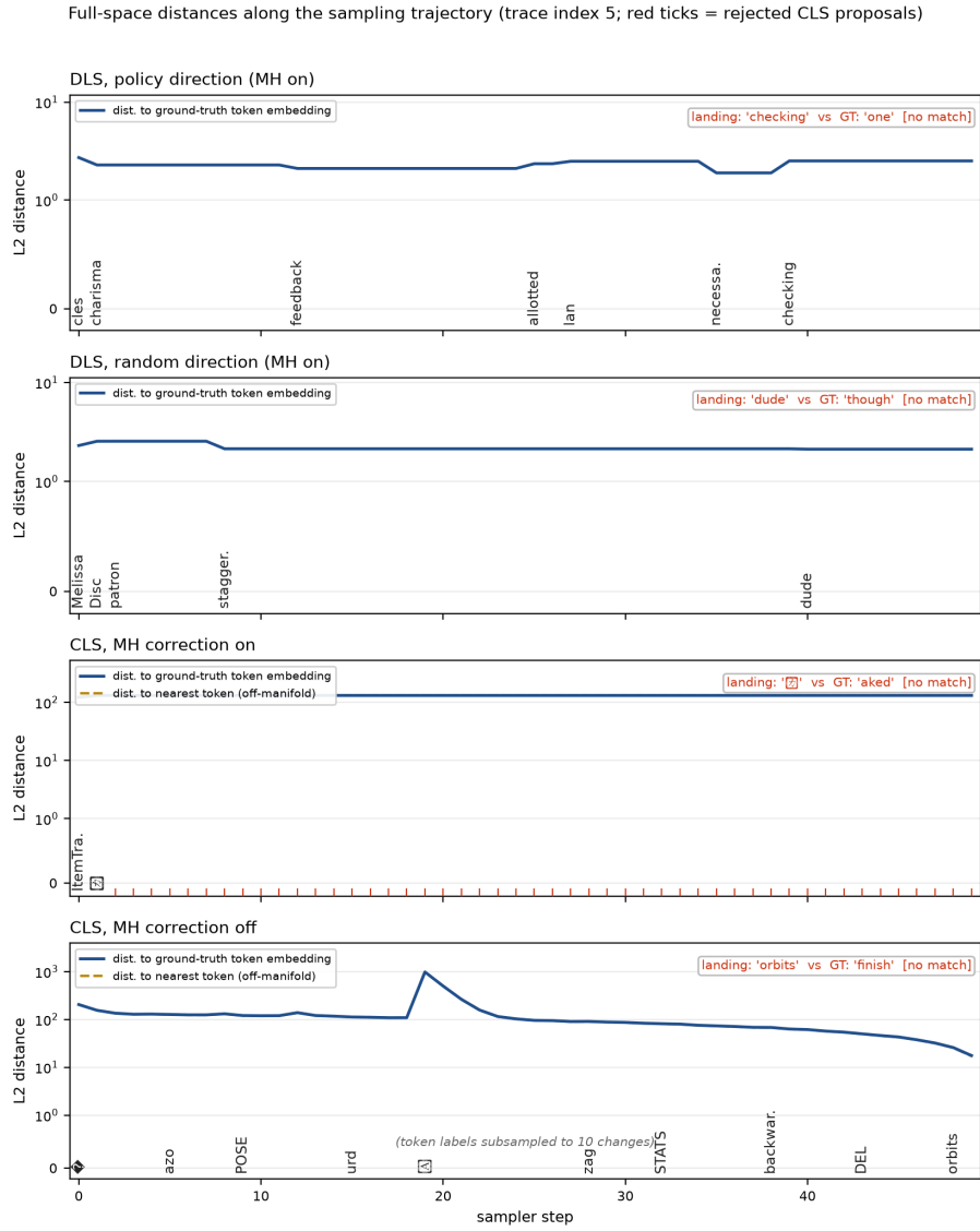
Figure 14: Full-space distances along the sampling trajectory for one trace, index 5, one panel per configuration.
