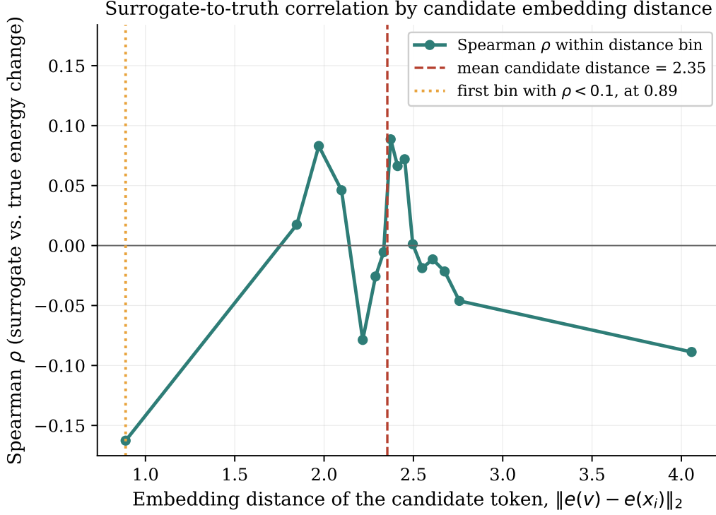
Figure 5: Correlation between the gradient surrogate and the true energy change as a function of the embedding distance of the candidate token, for GPT-2 Large.
