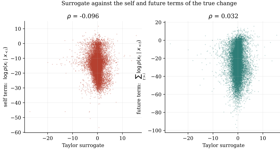
Figure 6: The true energy change decomposed into its self term and its future term, each plotted against the gradient surrogate, for GPT-2 Large.
