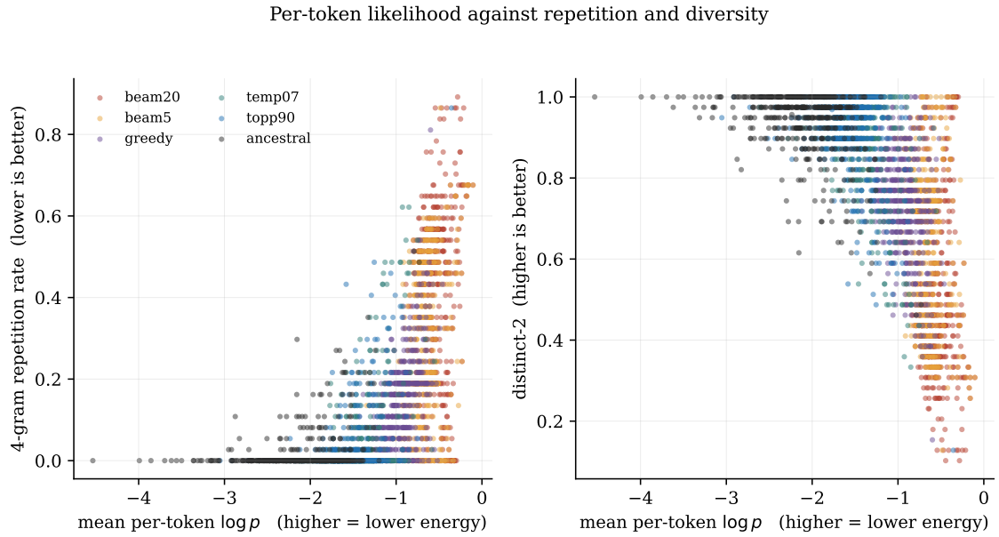
Figure 9: Mean per-token log-probability against 4-gram repetition rate and distinct-2 diversity for GPT-2 Large, one point per generation, coloured by decoding strategy.
