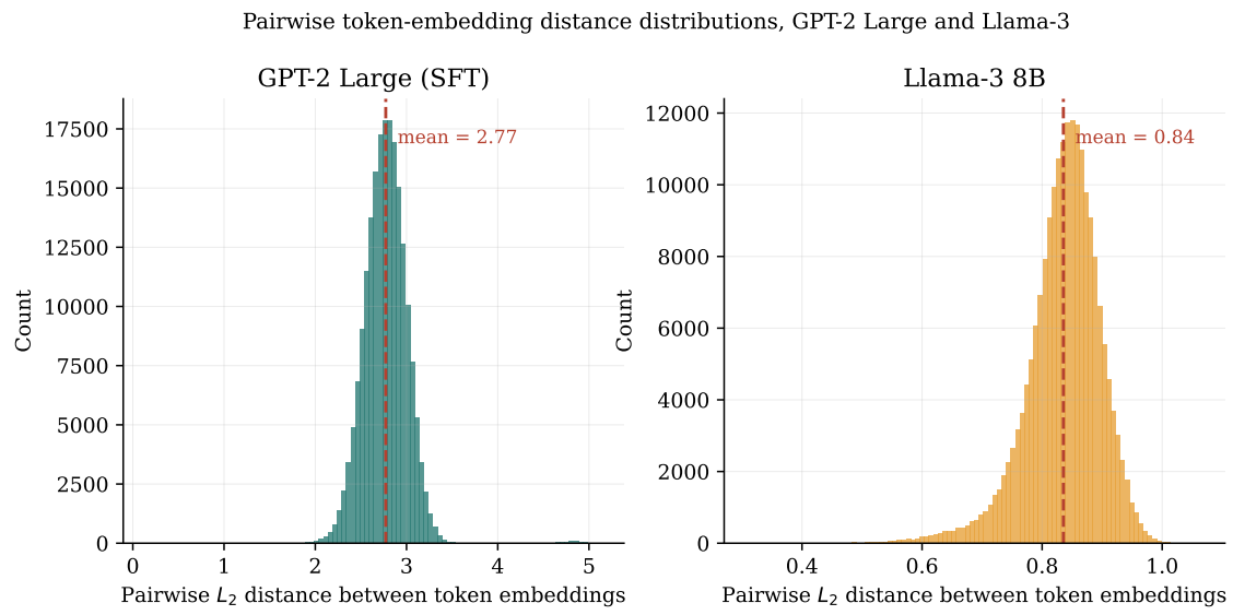
Figure 10: Distributions of pairwise token-embedding distances in GPT-2 Large and Llama-3, plotted on separate scales.
