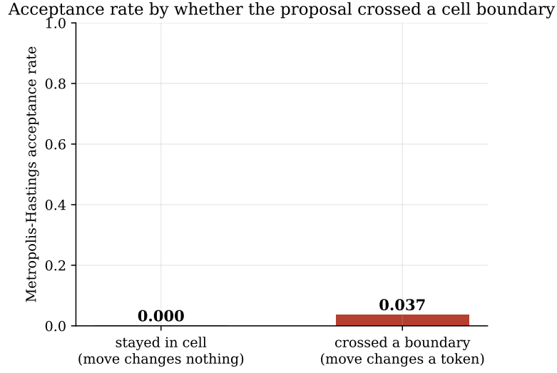
Figure 8: Metropolis–Hastings acceptance rate for the continuous policy sampler with gradient normalization off and the correction enabled, for that single configuration rather than pooled, conditioned on whether the proposal crossed a Voronoi cell boundary.
