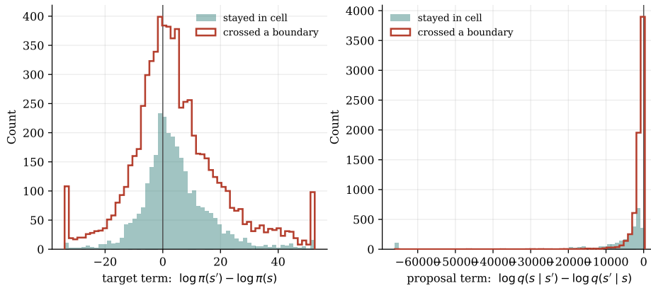
Figure 2: Decomposition of the Metropolis–Hastings acceptance ratio in the continuous sampler. Left: the target log-ratio. Right: the proposal log-ratio. Both on a log-probability scale.
