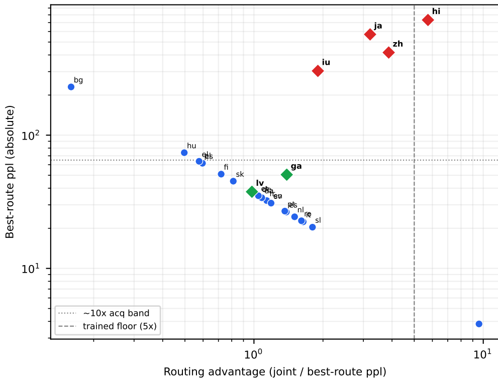
Two-axis OOD separation: 20 trained (blue) vs 6 unseen (diamonds)
