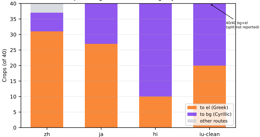
Cross-script routing concentrates on high-byte territories
