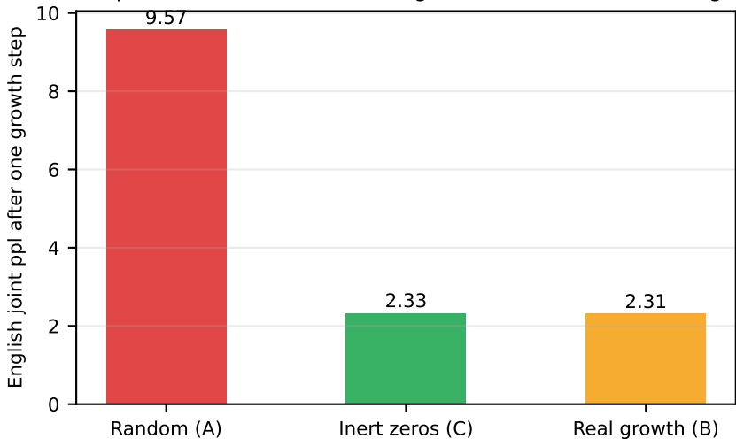
Expansion control: most damage is arithmetic, not learning
