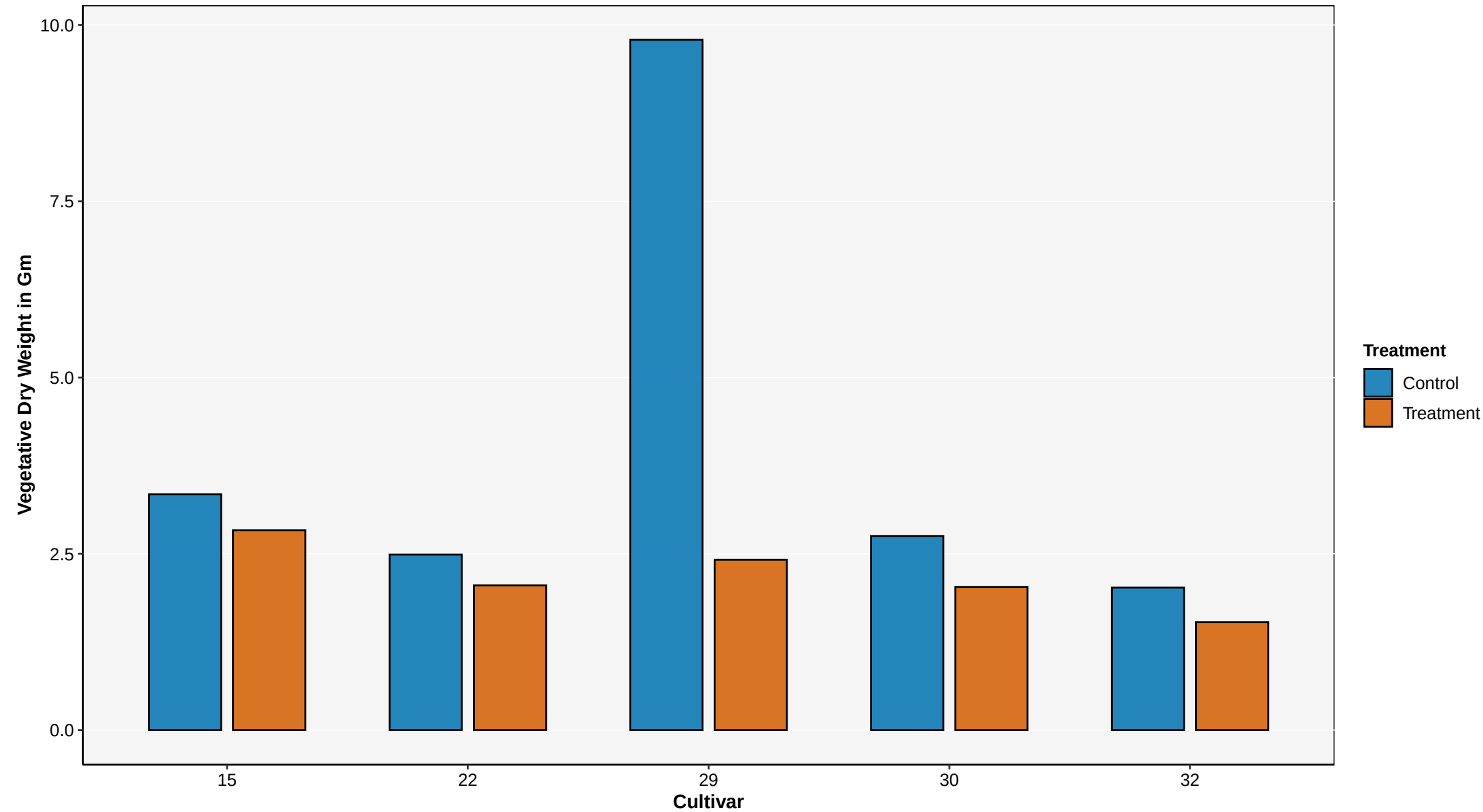
Mean of Replicates (All Timepoints Combined) – Vegetative Dry Weight in Gm
