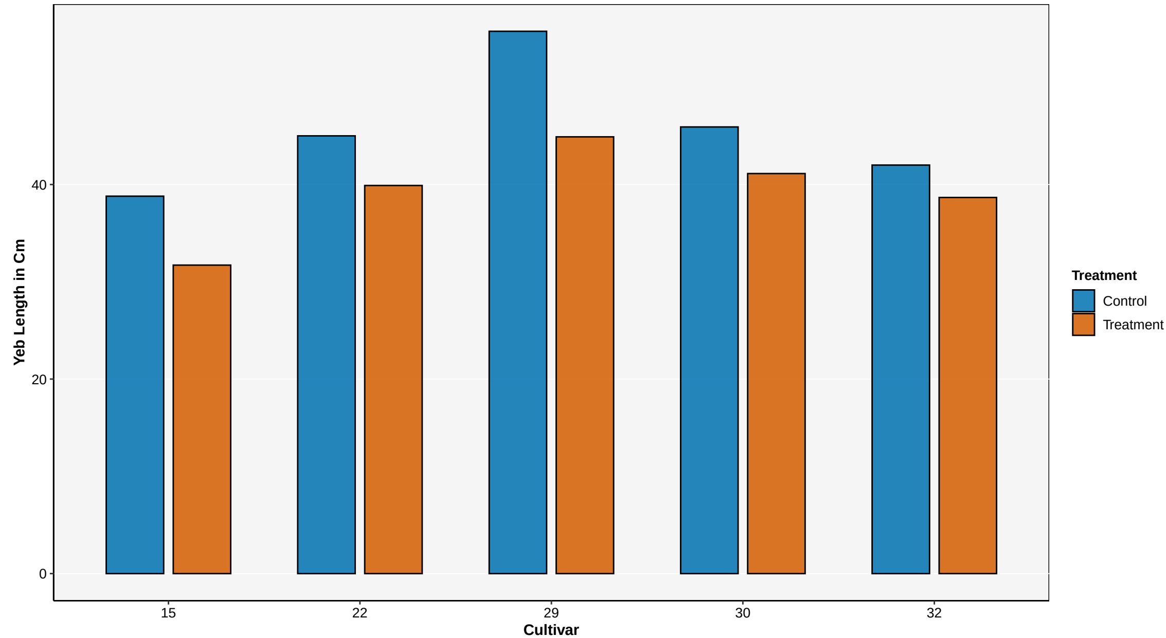
Mean of Replicates – Yeb Length in Cm (Timepoint 2)
