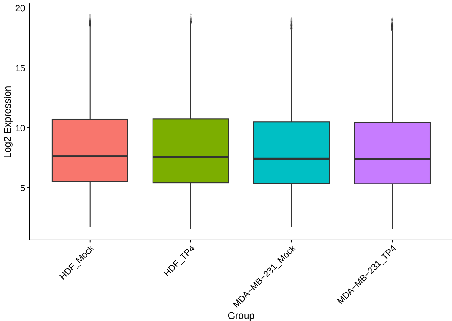
Expression Distribution by Group
