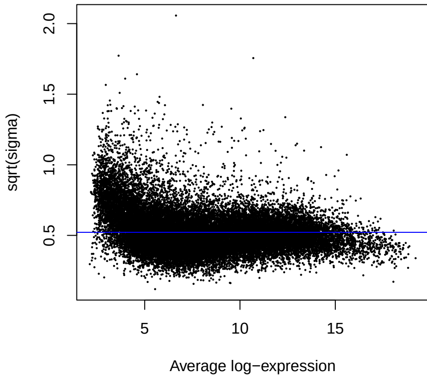
Mean-Variance Trend (after eBayes)
