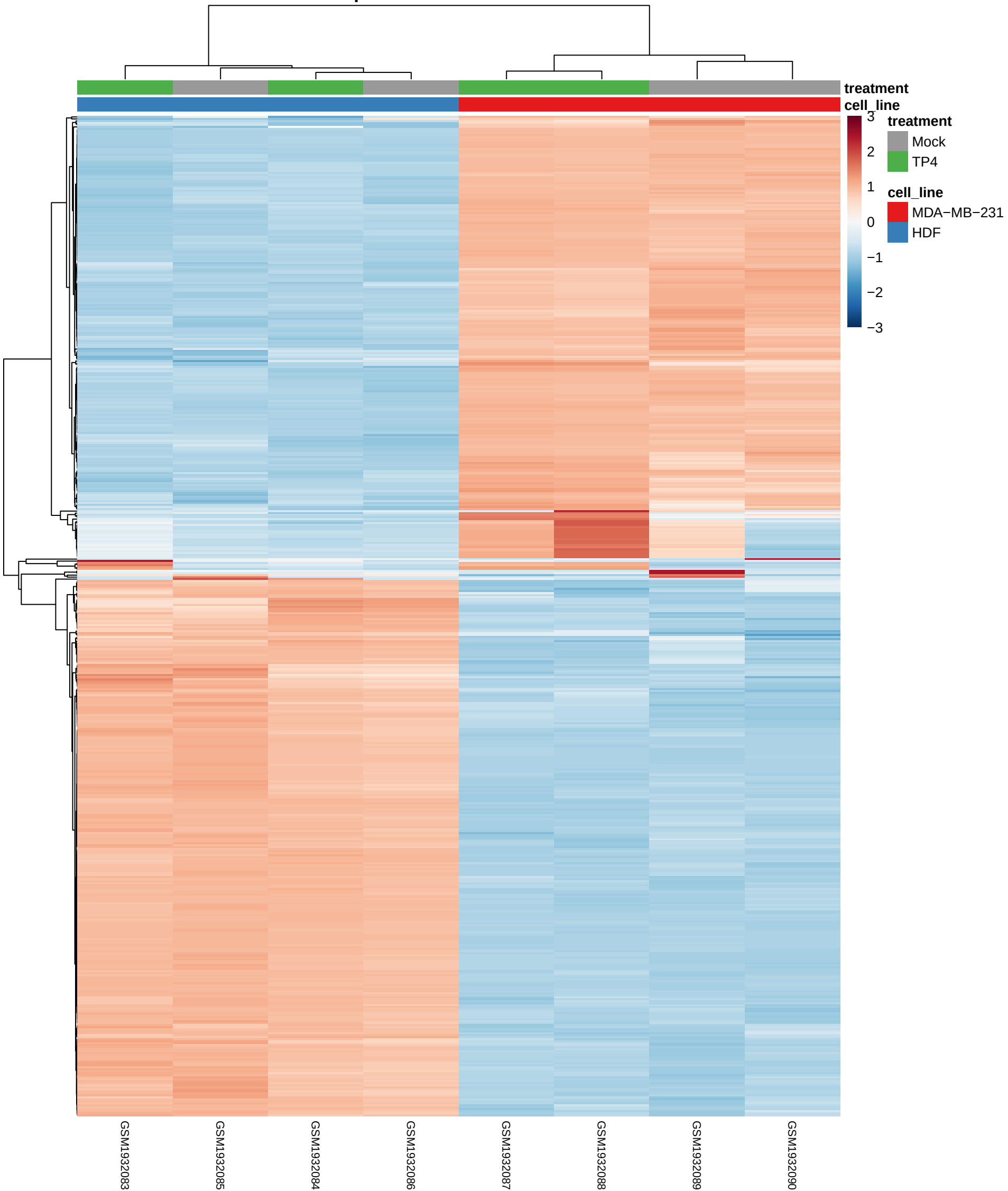
Top 500 Most Variable Genes
