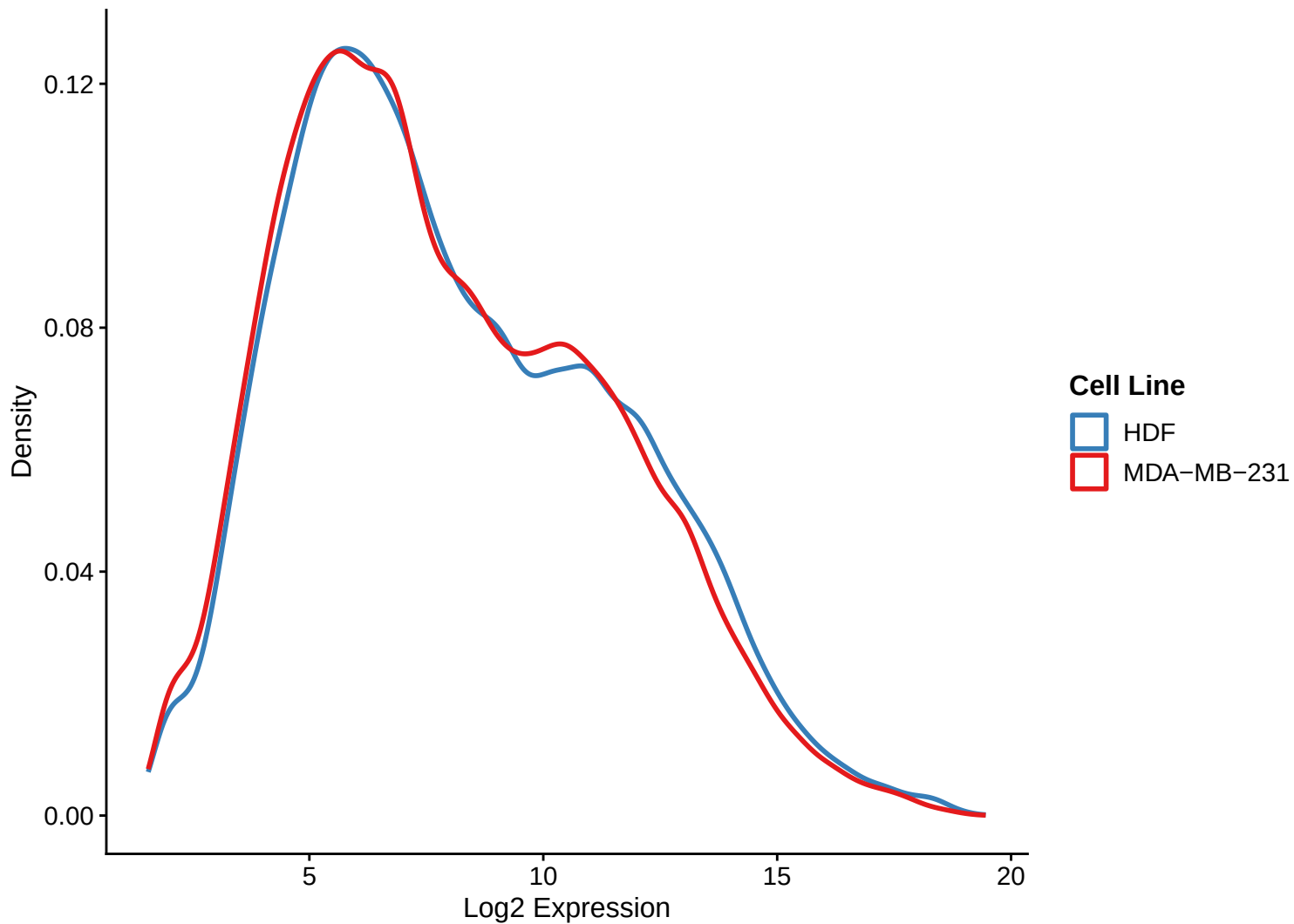
Expression Density Distribution by Cell Line
