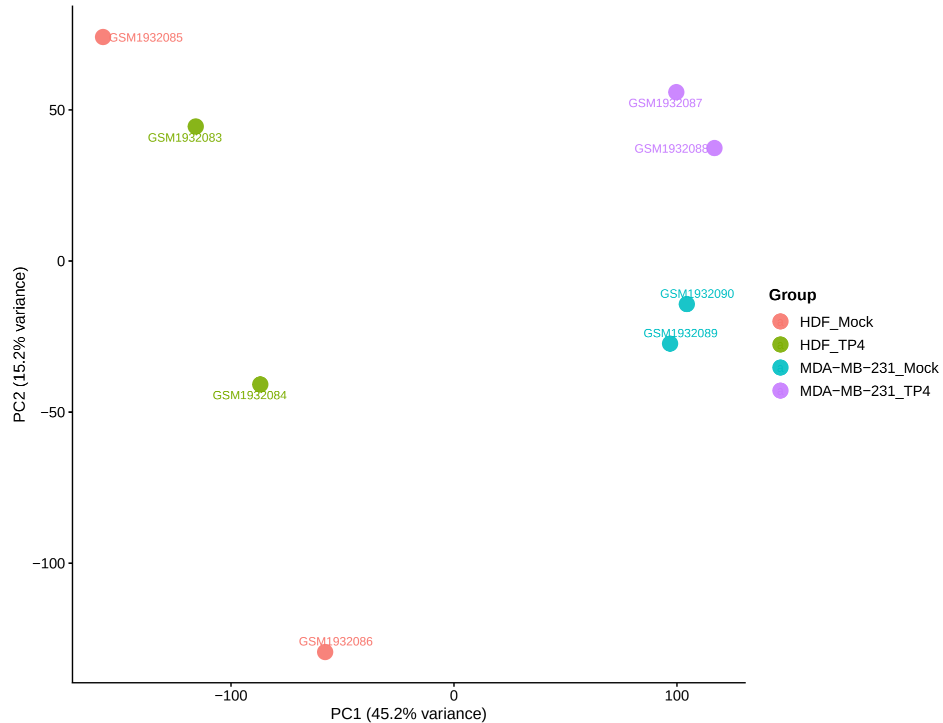
PCA of Gene Expression by Group
