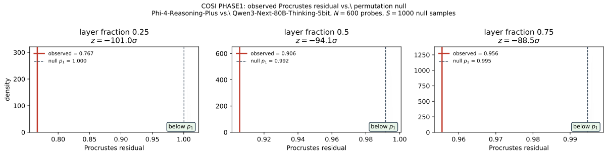
Figure 2: Phase 1 observed Procrustes residual (red vertical line) against the permutation null distribution (gray histogram; 200 samples shown for visualization, with summary statistics from the full S = 1000 run). Same caveats as Phase 0.
