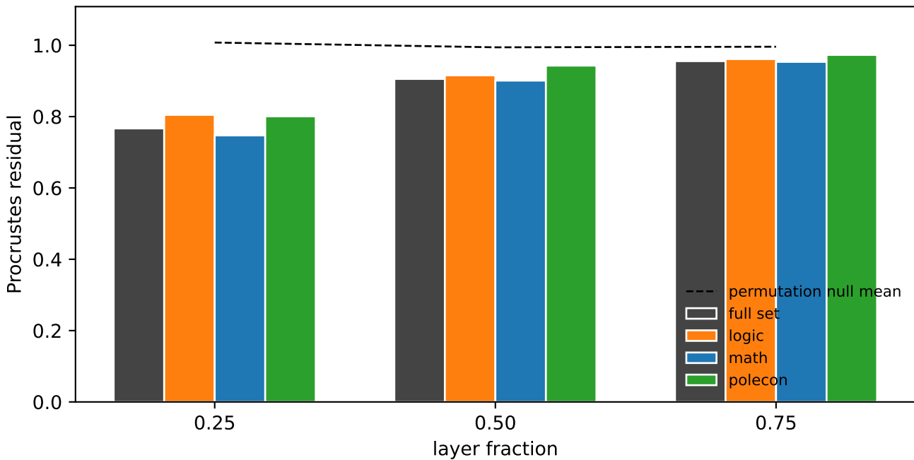
COSI PHASE1: alignment quality by domain Phi-4-Reasoning-Plus vs. Qwen3-Next-80B-Thinking-5bit
