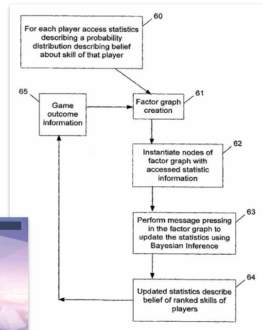
TrueSkill | WO2007094909A1
