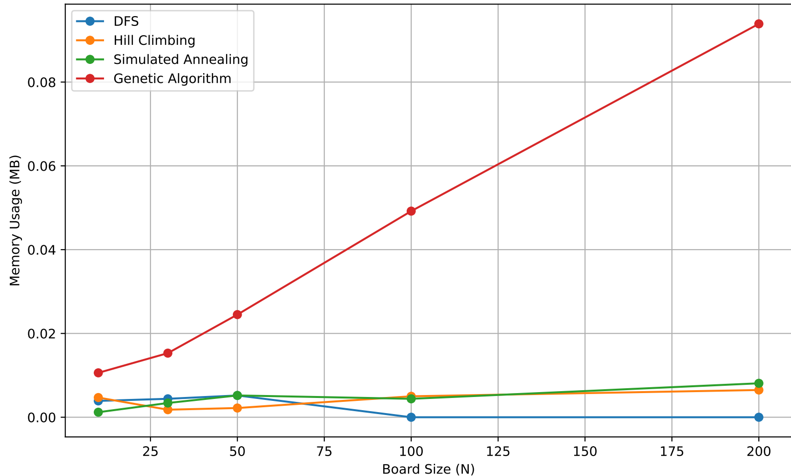
Memory Usage Comparison of N-Queens Algorithms
