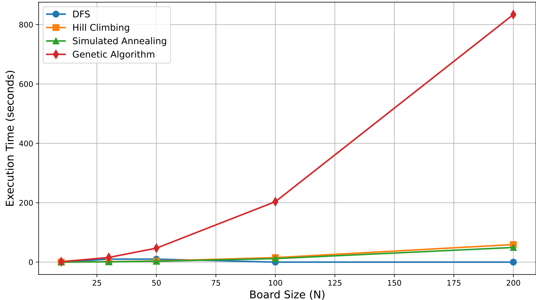
Execution Time Comparison of N-Queens Algorithms
