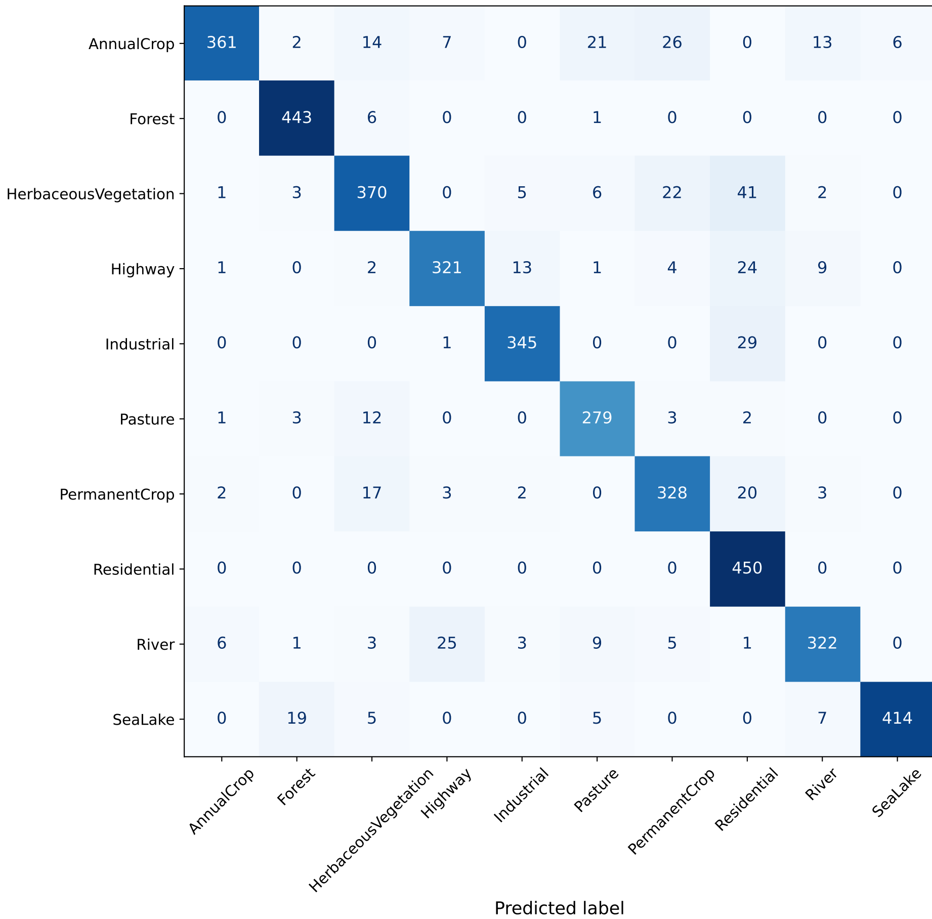
Confusion Matrix - Custom CNN
