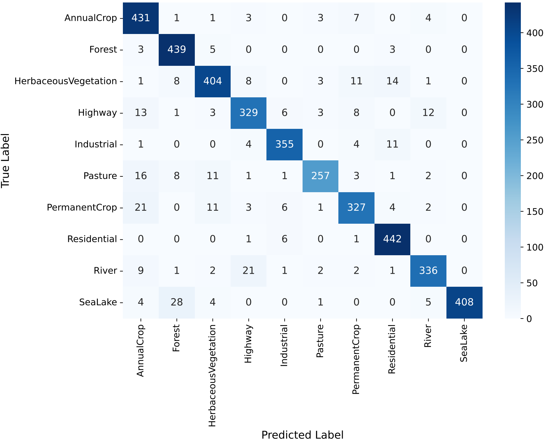
EfficientNetB0 Confusion Matrix
