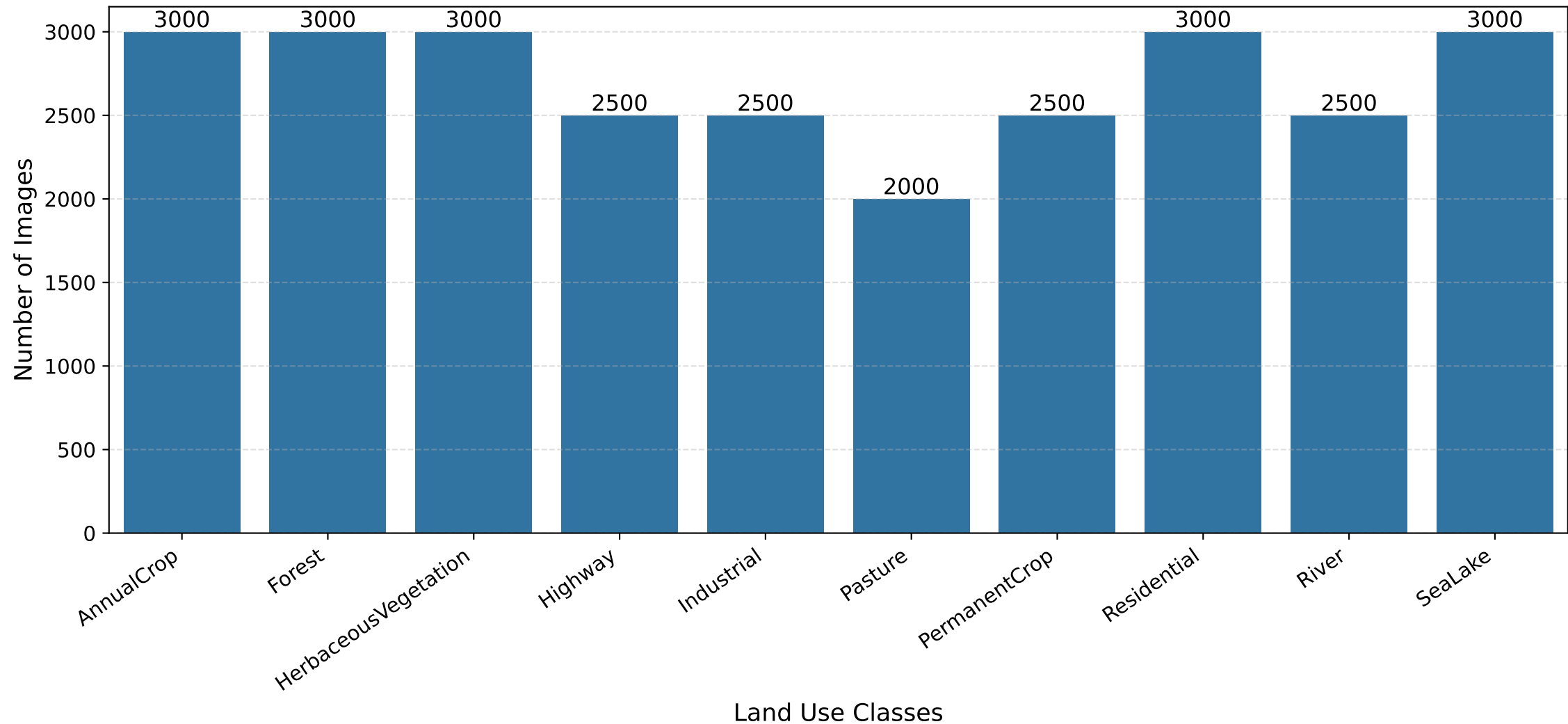
Class Distribution of the EuroSAT RGB Dataset
