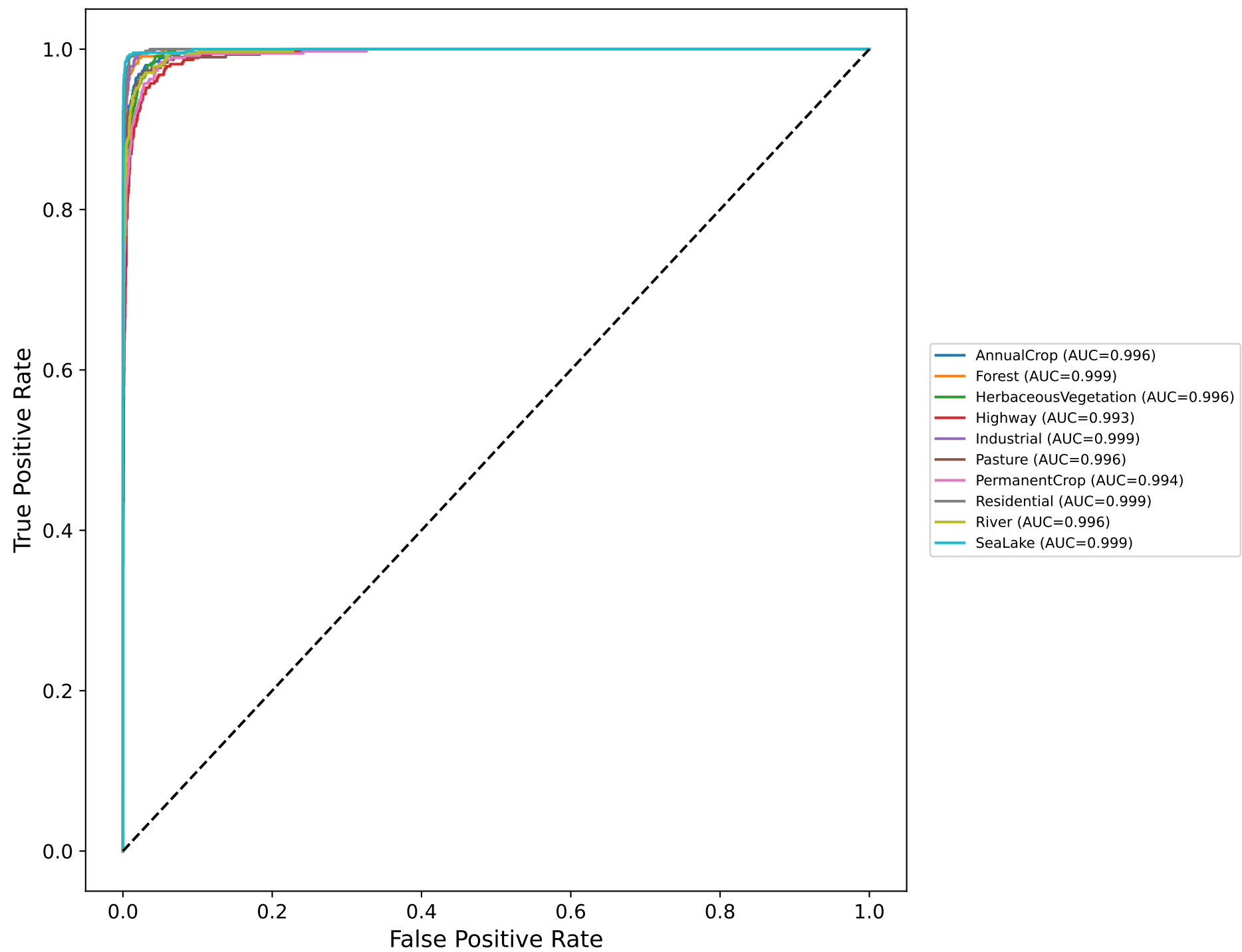
EfficientNetB0 ROC Curves
