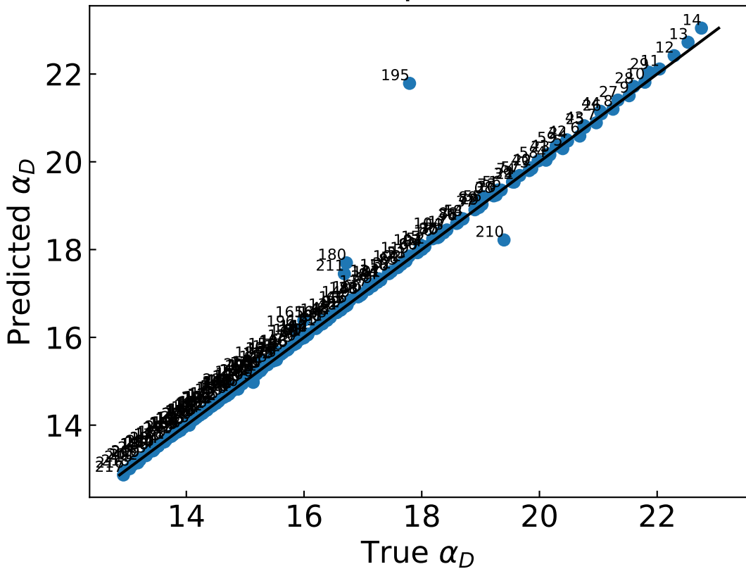
Main branch \alpha_D : prediction vs truth
