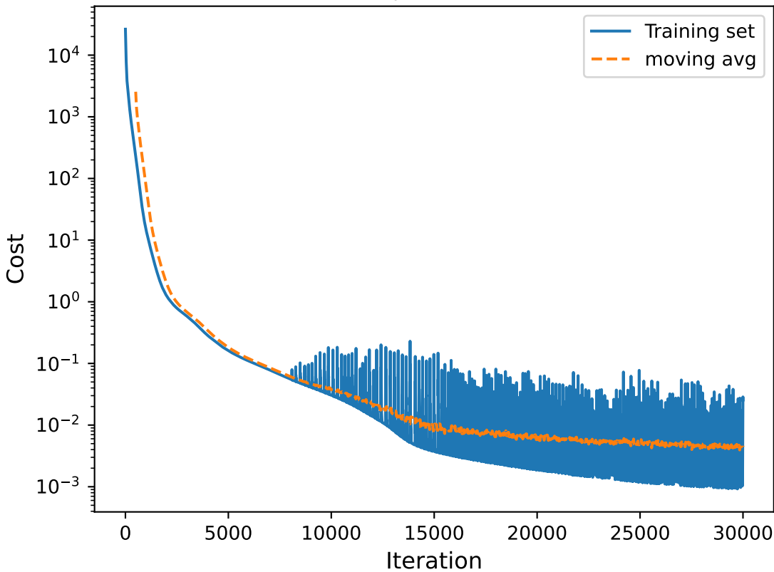
Cost history (seed=44) | best=9.220e-04 @ iter 29729
