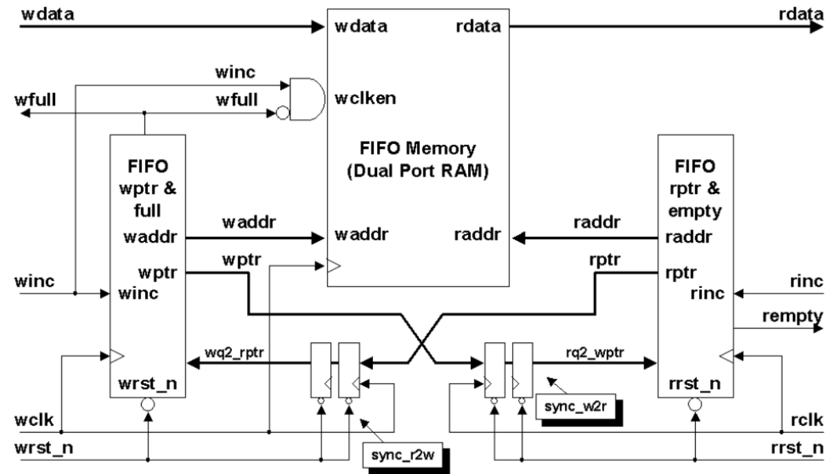
Figure 5 - FIFO01 partitioning with synchronized pointer comparison
