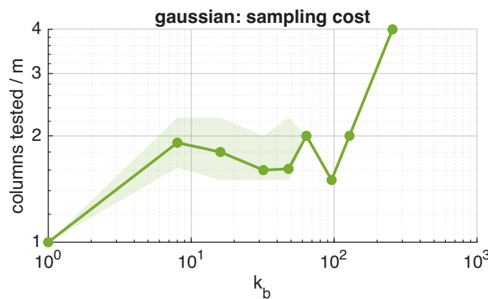
Effect of block size on norm-weighted sampling ( m=64 )
