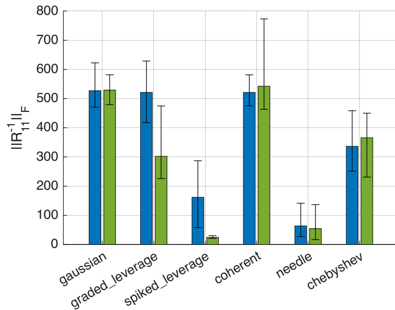
Uniform vs norm-weighted sampling ( m=64 , n=32000 , k_b=64 )
