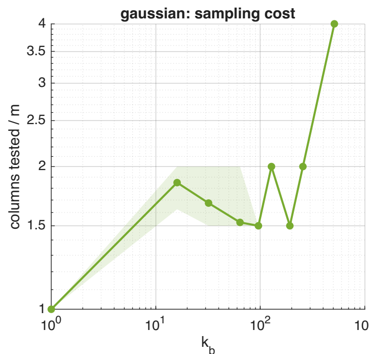
Effect of block size ( m=128 , n=8000 )
