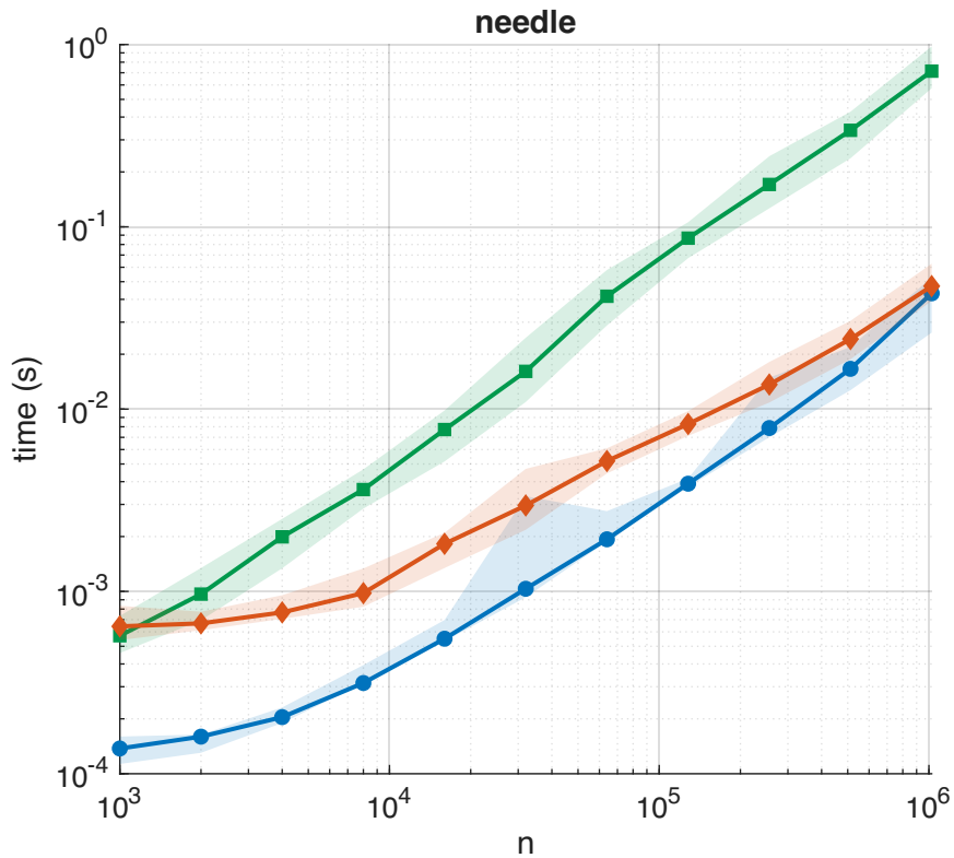
Runtime vs n at fixed m = 64
