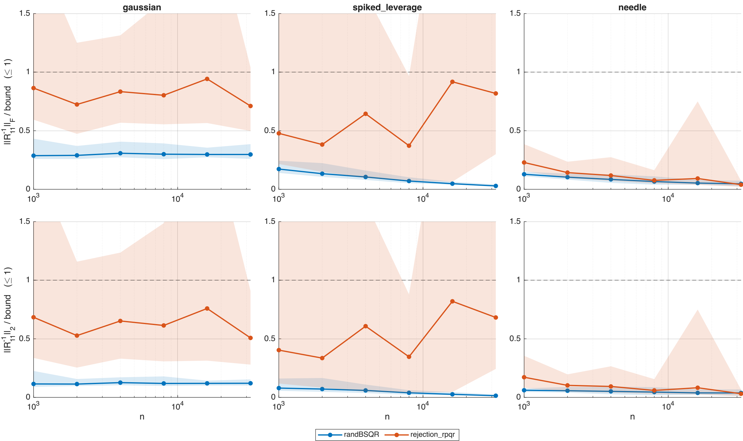
Selection quality vs bounds (m=256)
