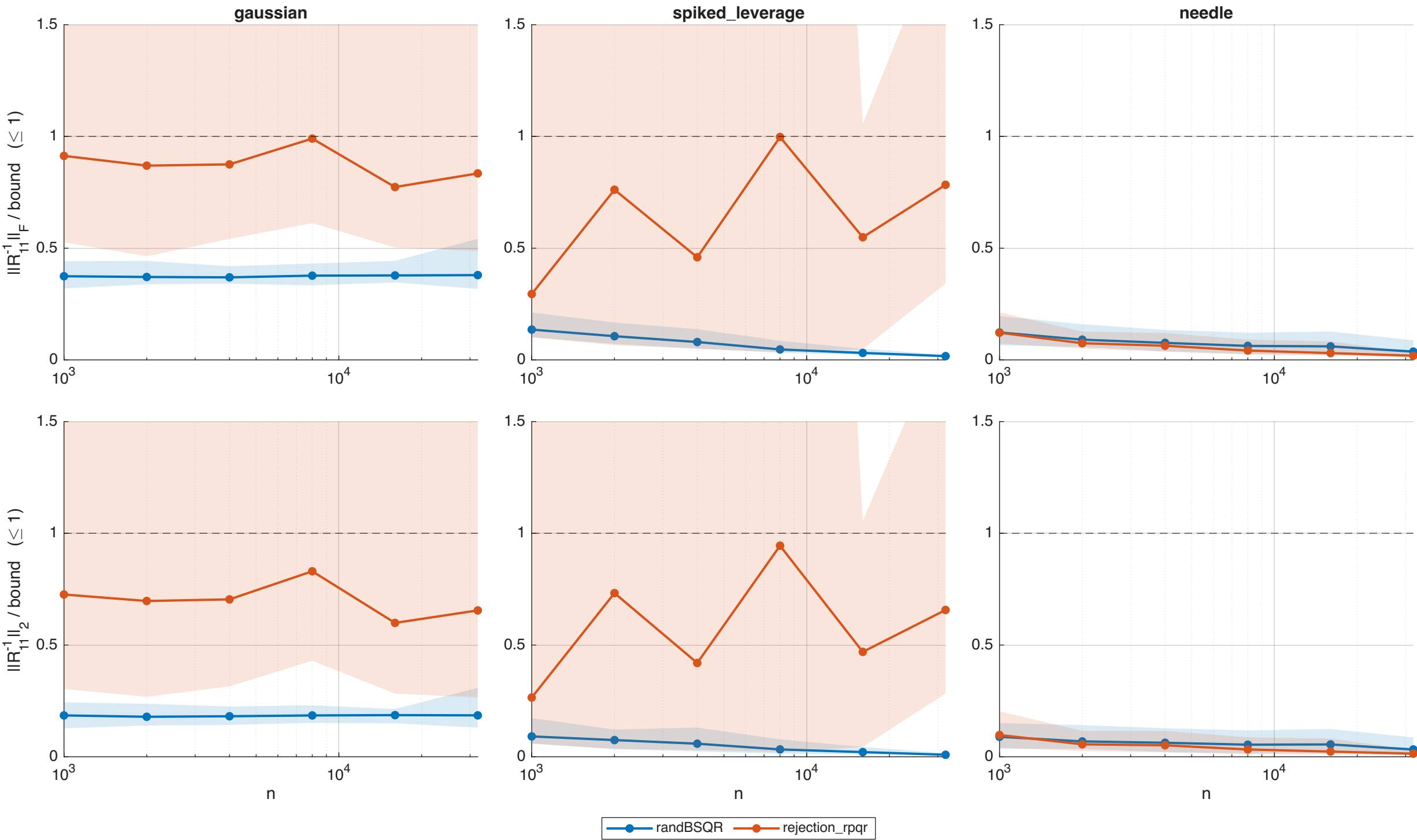
Selection quality vs bounds (m=64)
