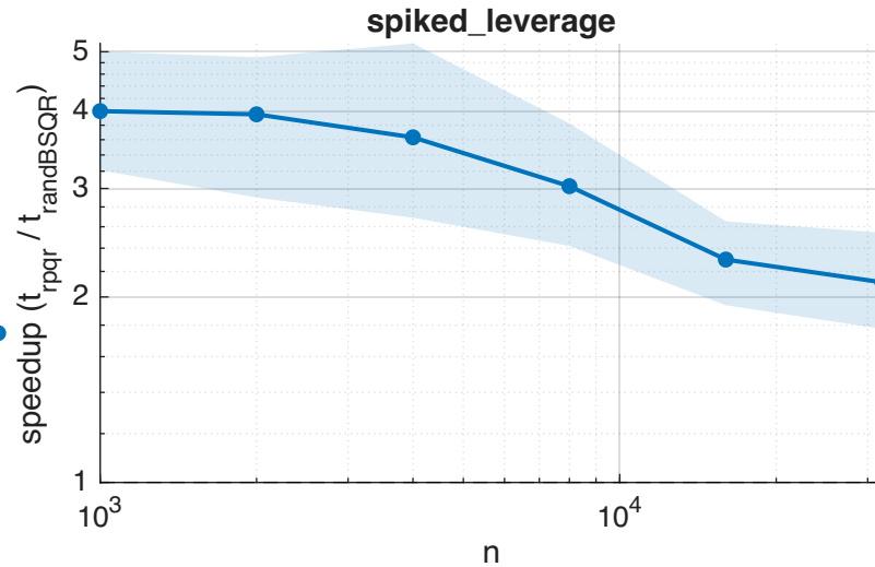
Speedup of randBSQR over rejection_rpqr (m=128)
