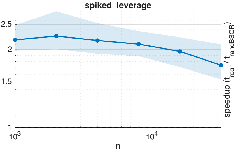
Speedup of randBSQR over rejection_rpqr (m=256)
