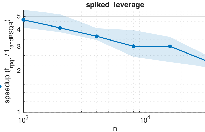
Speedup of randBSQR over rejection_rpqr (m=64)
