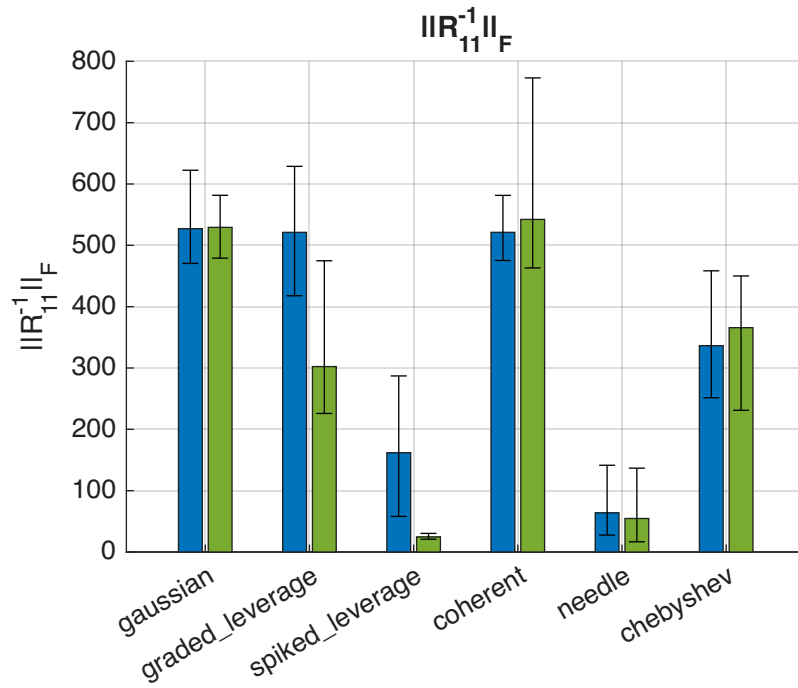
Uniform vs norm-weighted sampling ( m=64 , n=32000 , k_b=64 )
