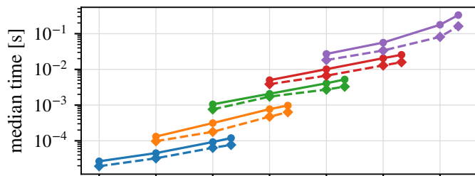
Gaussian — 1 thread
