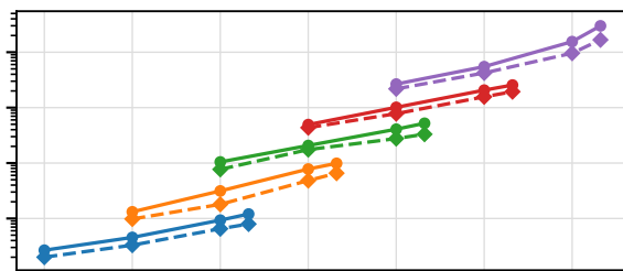
Ill-conditioned — 4 threads
