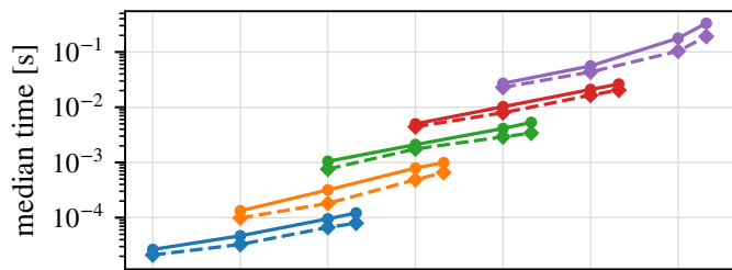
Ill-conditioned — 1 thread
