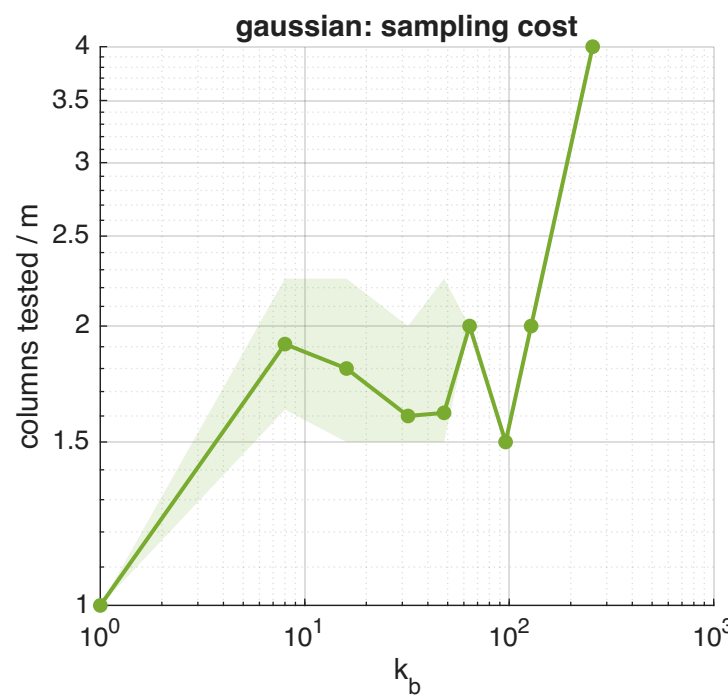
Effect of block size ( m=64 , n=8000 )
