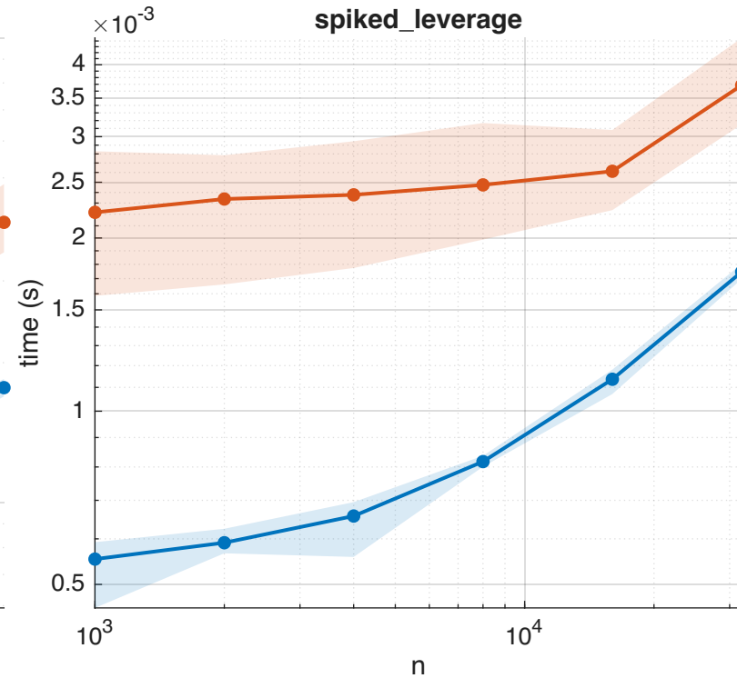
Runtime vs n (m=128)
